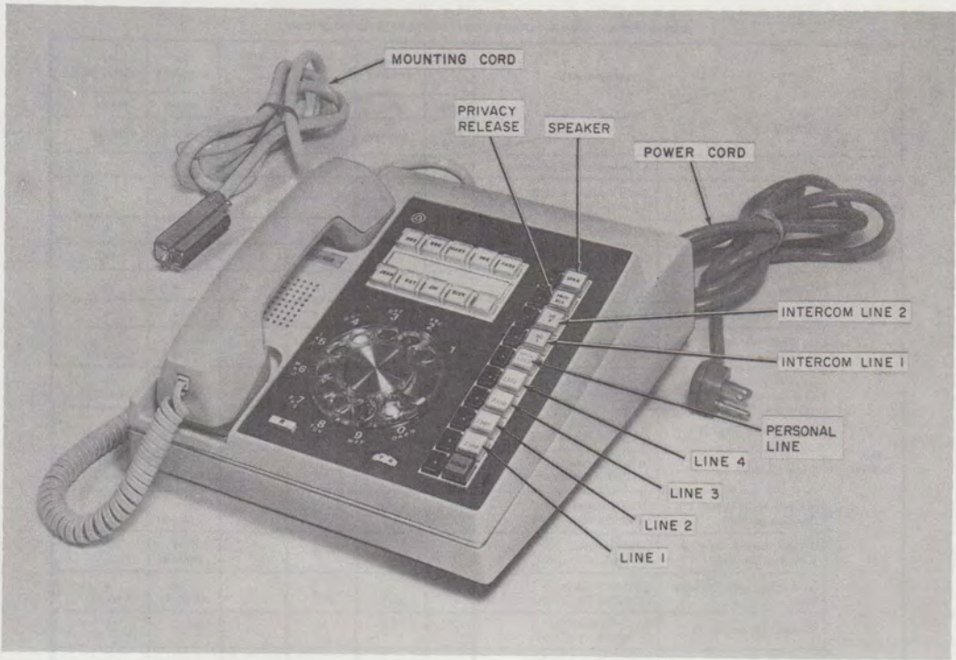
Fig. 1—Primary Telephone Set
