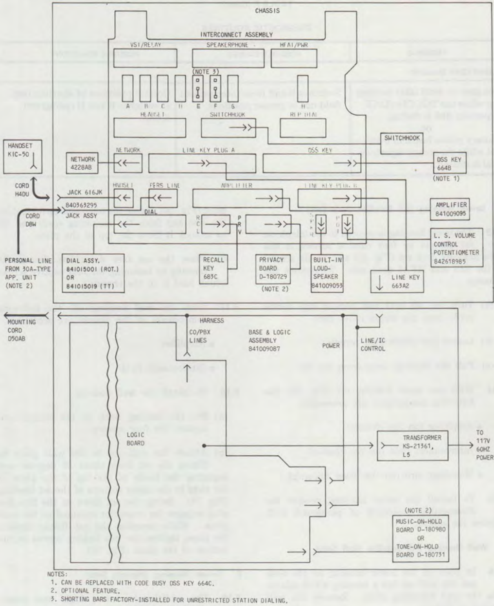
Fig. 48—Block Diagram of Primary Set
