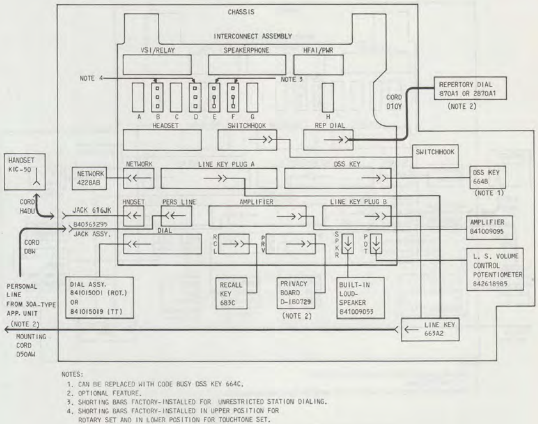
Fig. 49—Block Diagram of Basic Satellite Desk Set
