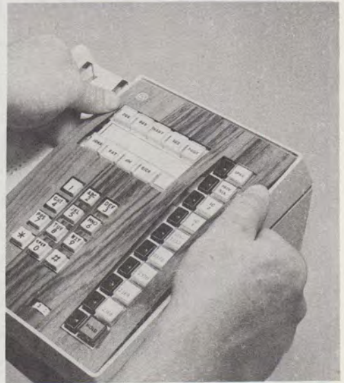
Fig. 54—Installing Faceplate
