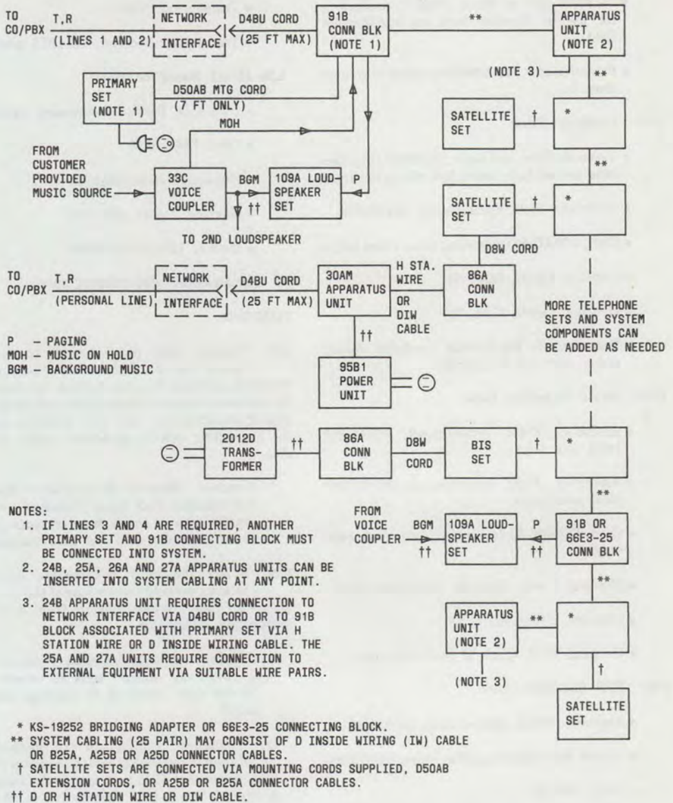
Fig. 9—Typical Installation Using Bridged Connections
