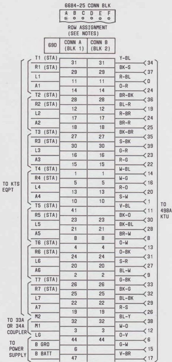
Fig. 35.1—Nondedicated Lead Connections for 498A KTU (Music-On-Hold Circuit) Equipped With a 116A1 Circuit Module in 69D Apparatus Mounting
