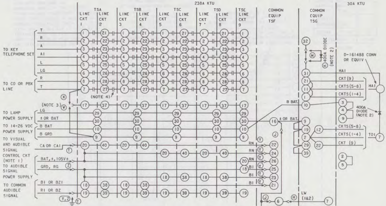
Fig. 4—Connections for CO or PBX Line Circuits (238A KTU) with 30A and 227B KTUs for Line Pickup and Hold, Line and Busy Lamps, Interrupted Audible Signals, Common Audible Signals, Auxiliary Timeout, and Lamp Wink (Sheet 1)
