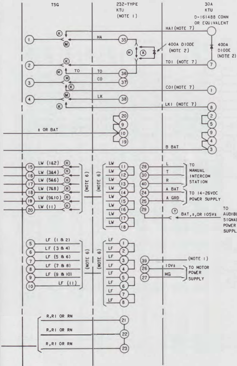
Fig. 6—Connections for CO or PBX Line Circuits (239A KTU) with 232-Type, 30A, and 227B KTUs for Line Pickup and Hold, Line and Busy Lamps, Interrupted Audible Signals, Common Audible Signals, Auxiliary Timeout, Lamp Wink, and Manual Intercom (Sheet 2)
