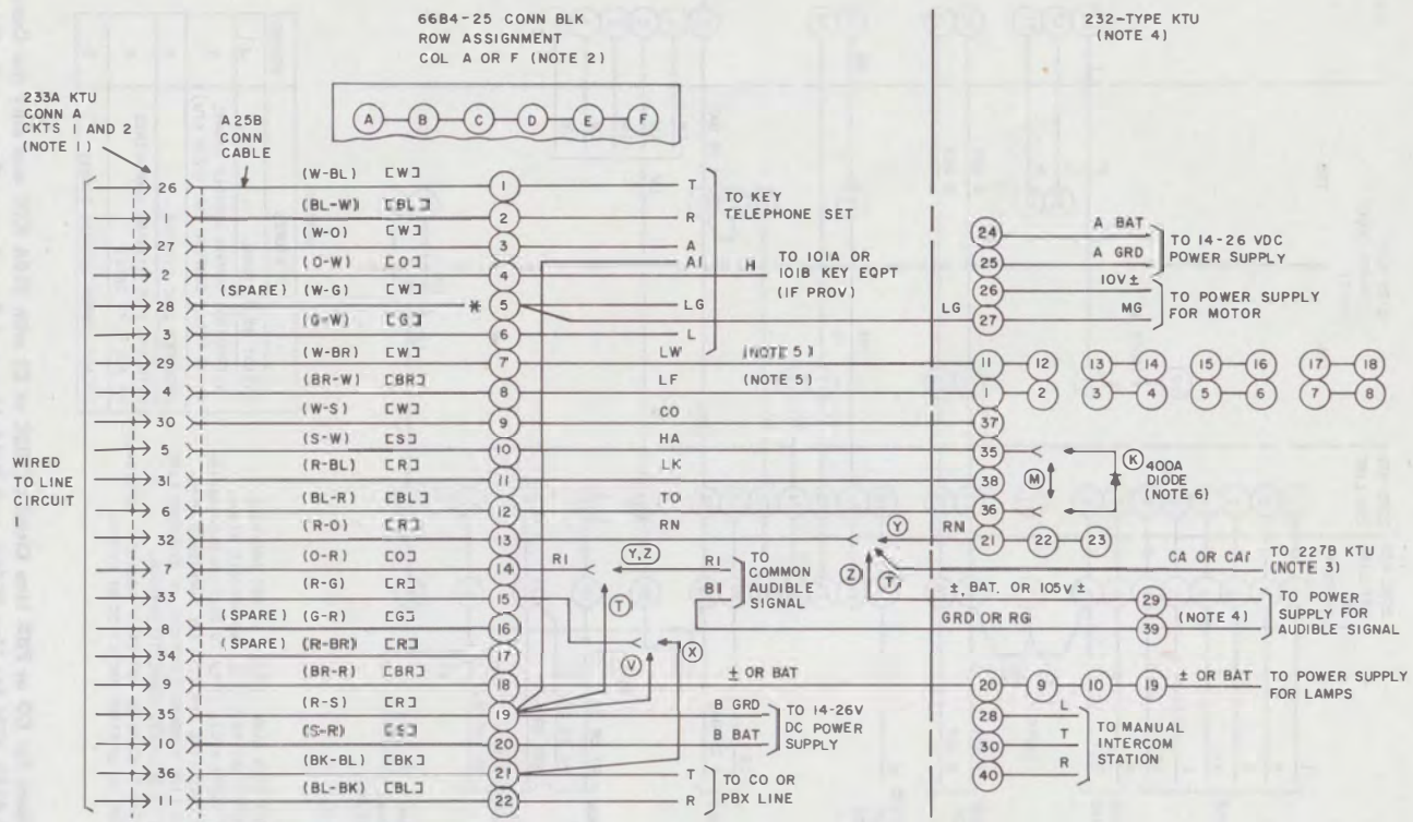
Fig. 9 —Connections for CO or PBX Line Circuits (233A KTU) with 227B and 232-Type KTUs for Line Pickup and Hold, Line and Busy Lamps, Interrupted Audible Signals, Lamp Wink, Manual Intercom, and Timeout (Sheet 1)
