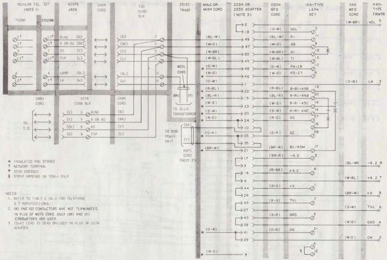
Fig. 4—Typical Grandfathered 4A Speakerphone System Arrangement, Connections to 702BM and 2702BM Telephone Sets
