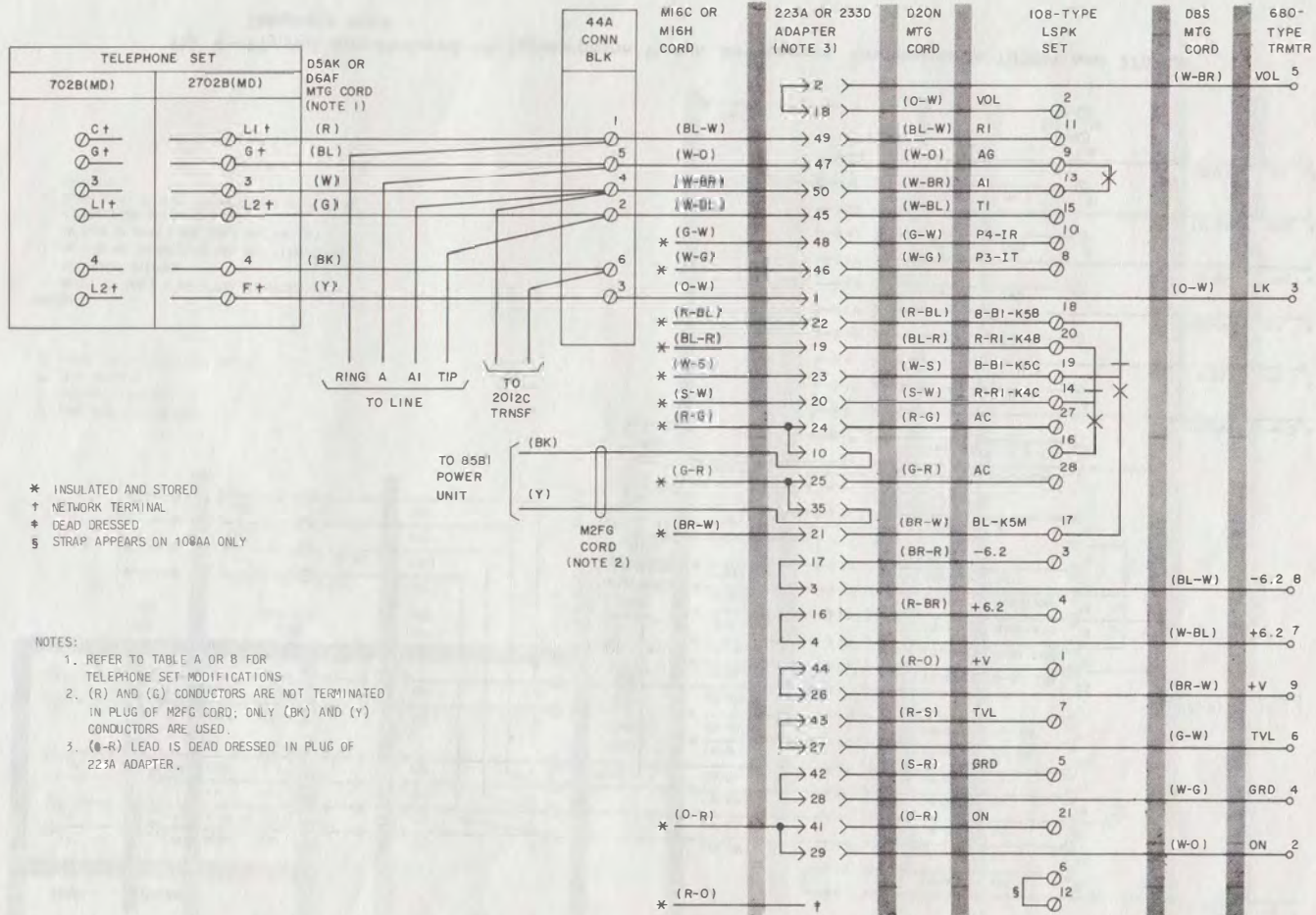
Fig. 3—Typical Grandfathered 4A Speakerphone System Arrangement, Connections to 702B (MD) and 2702B (MD) Telephone Sets
