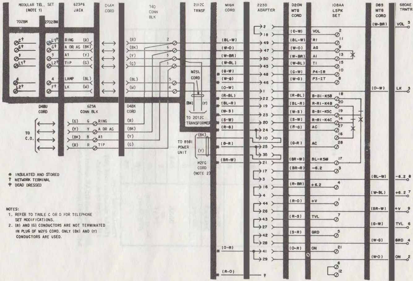
Fig. 5—Registered 4A Speakerphone System Arrangement, Connections to 702BM and 2702BM Telephone Sets
