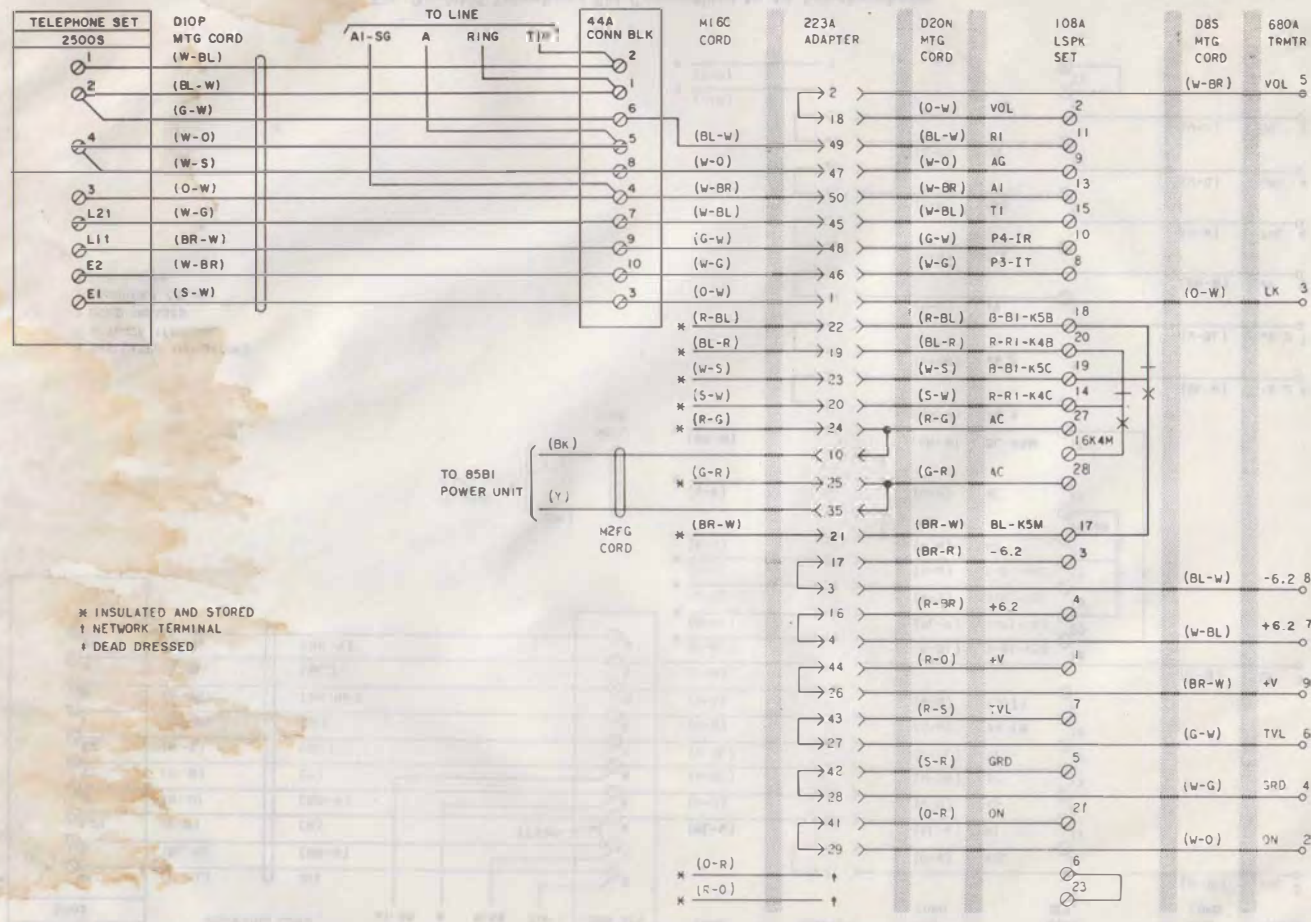
Fig. 3—2500S Telephone Set, Connections to 4A Speakerphone
