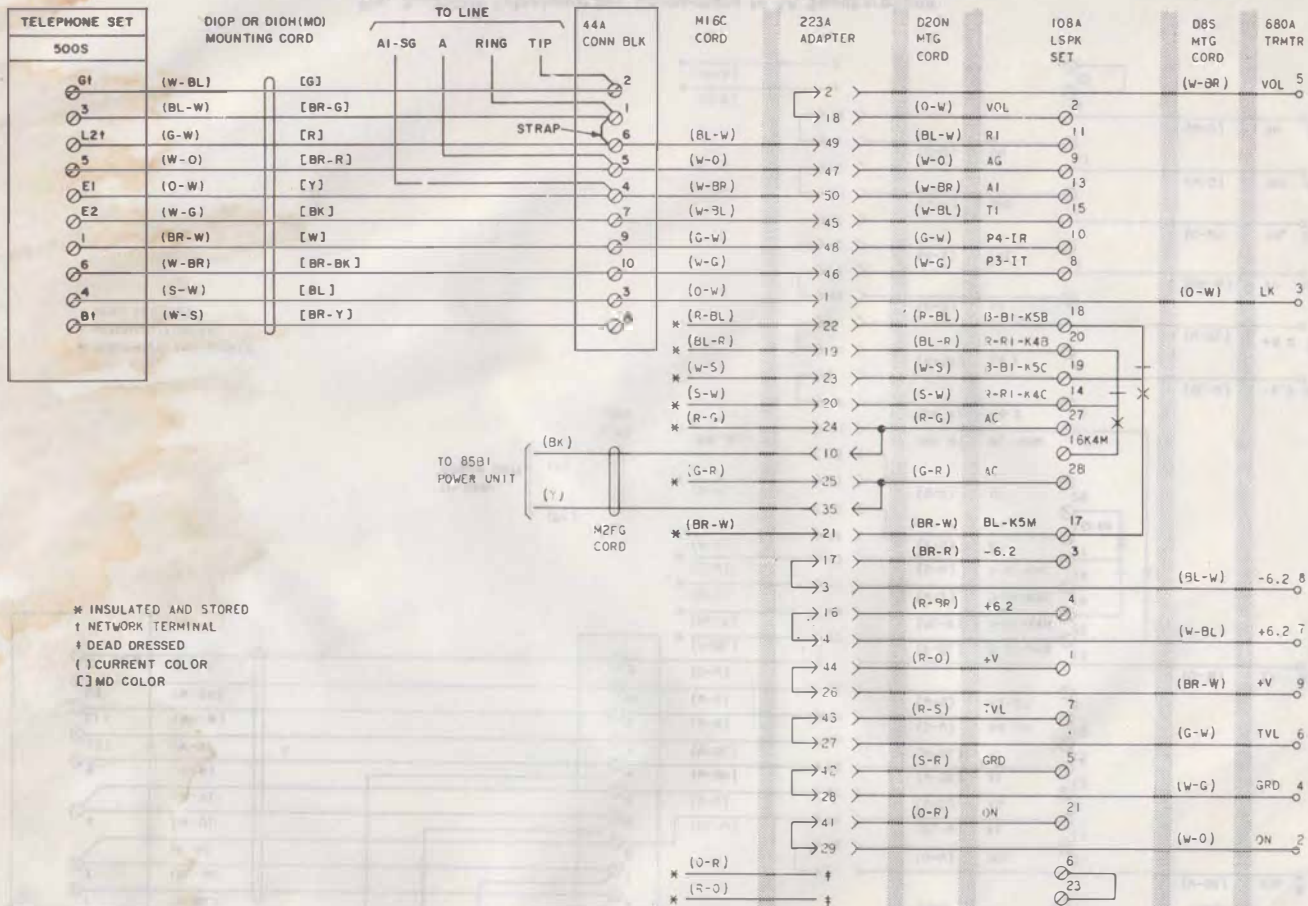
Fig. 2—500S Telephone Set Connections to 4A Speakerphone
