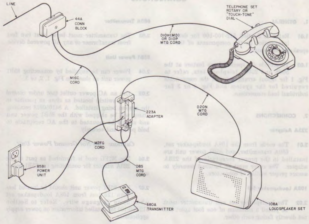
Fig. 1—Speakerphone Arrangement, 5005 or 25005 Telephone Set
