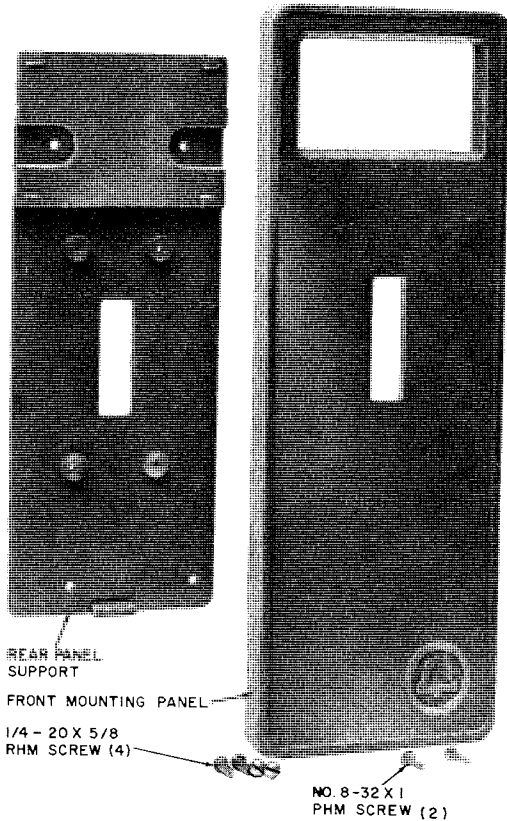
Fig. 9—KS-22284 Backboard
