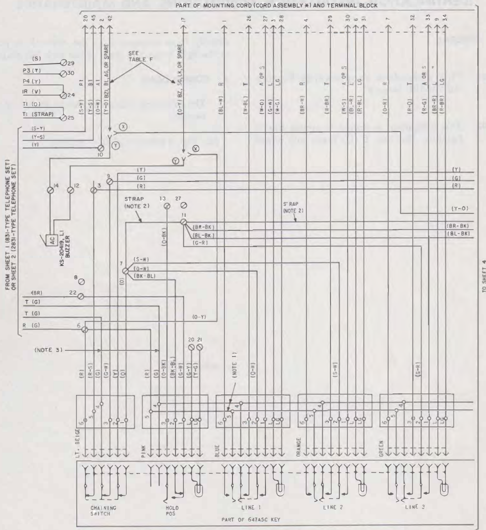
Fig. 9—831- and 2831-Type Telephone Set, Connections (Sheet 3 of 6)
