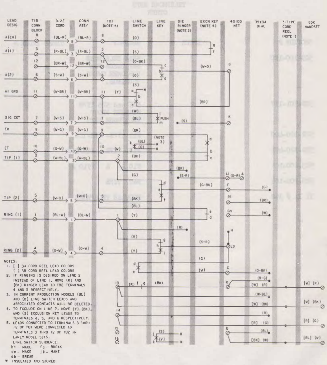
Fig. 1—2751C and D Telephone Sets, Connections
