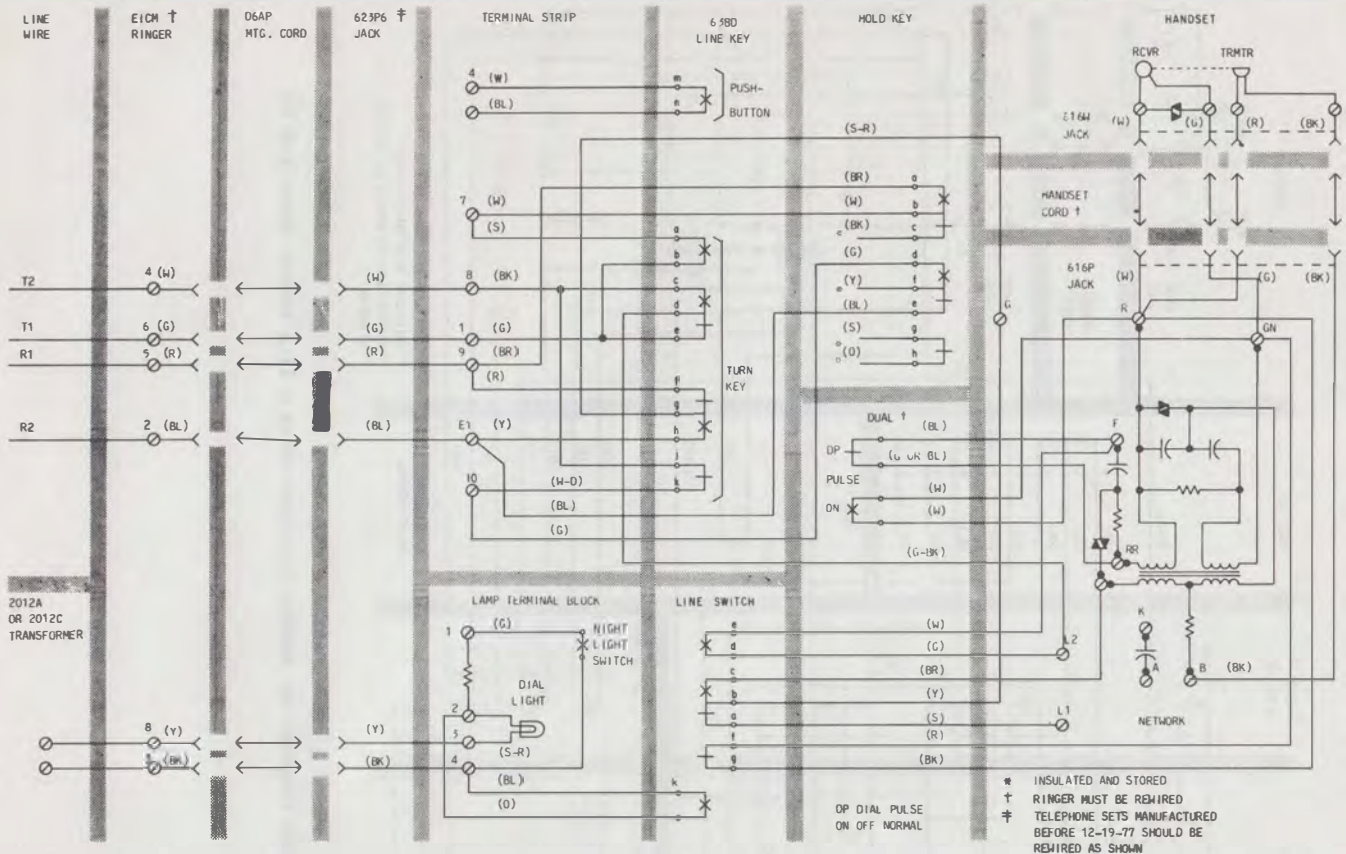
Fig. 3—713BM Telephone Set, Modular Connections Using a E1CM Ringer
