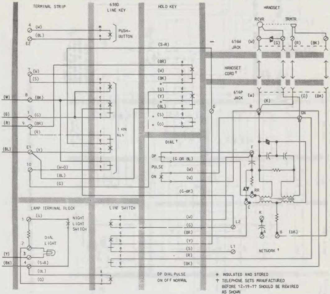
Fig. 2—281A Telephone Set, Modular Connections Using a 281A Adapter (Sheet 2 of 2)
