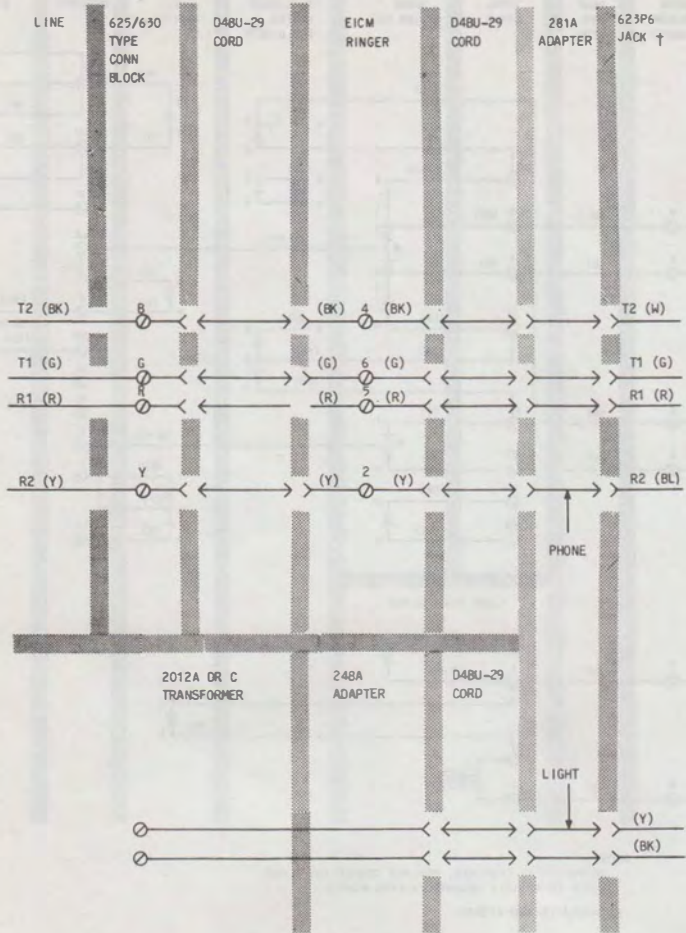
Fig. 2—713BM Telephone Set, Modular Connections Using a 281A Adapter (Sheet 1 of 2)
