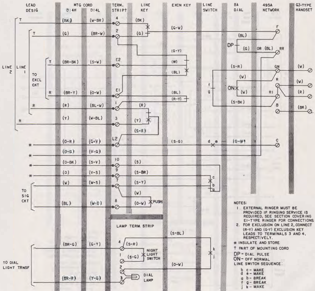
⚡ Fig. 1—711B (MD) Telephone Set Connections wired for 2-Line Pickup, Exclusion on Line 1 ⚡
