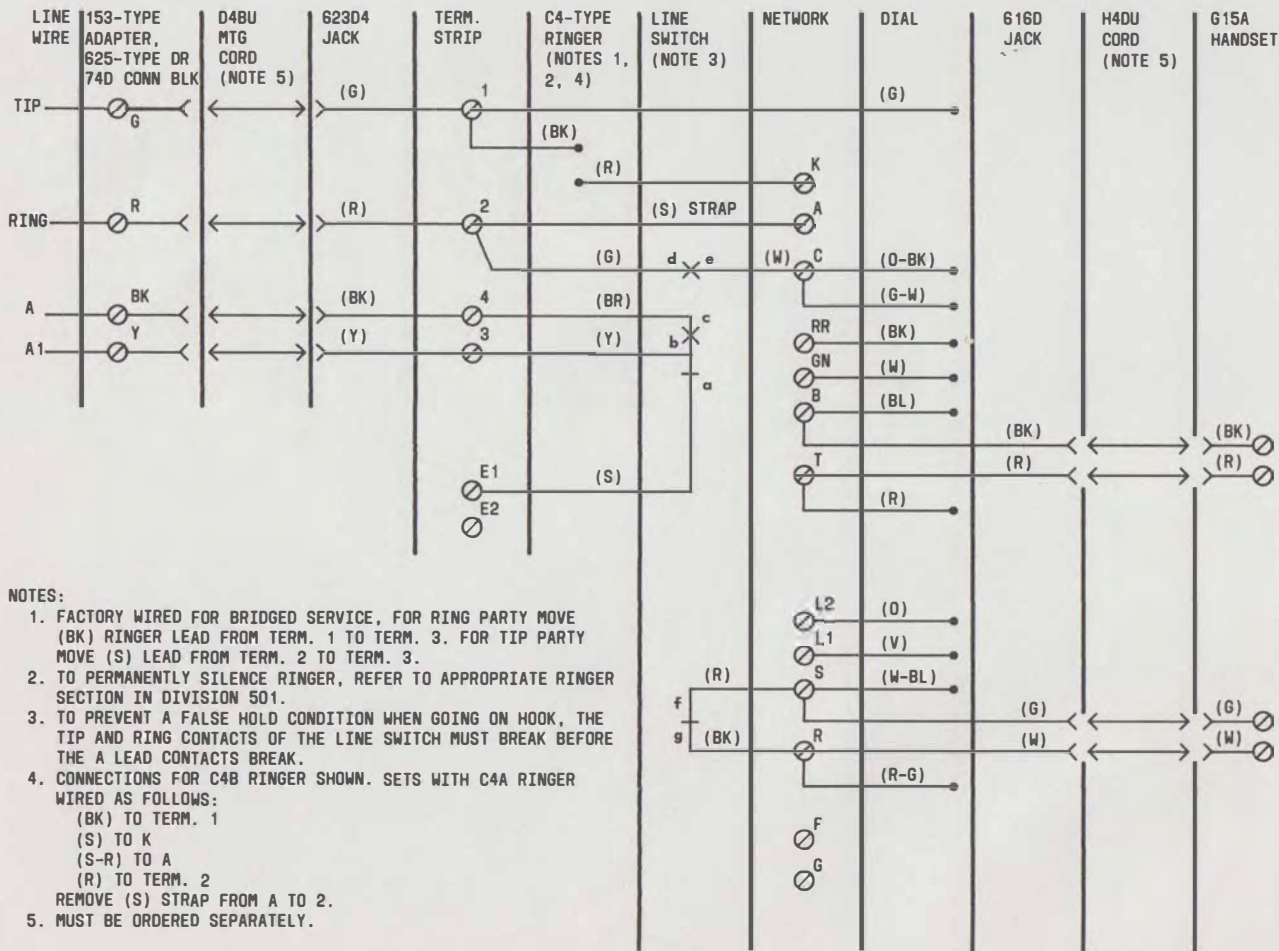
Fig. 2—2500SM Telephone Set, Connections
