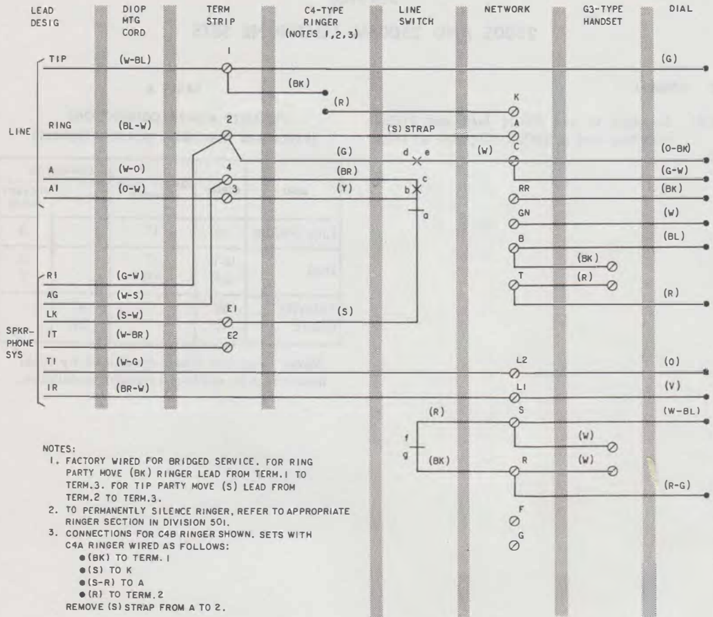
Fig. 1—2500S Telephone Set, Connections
