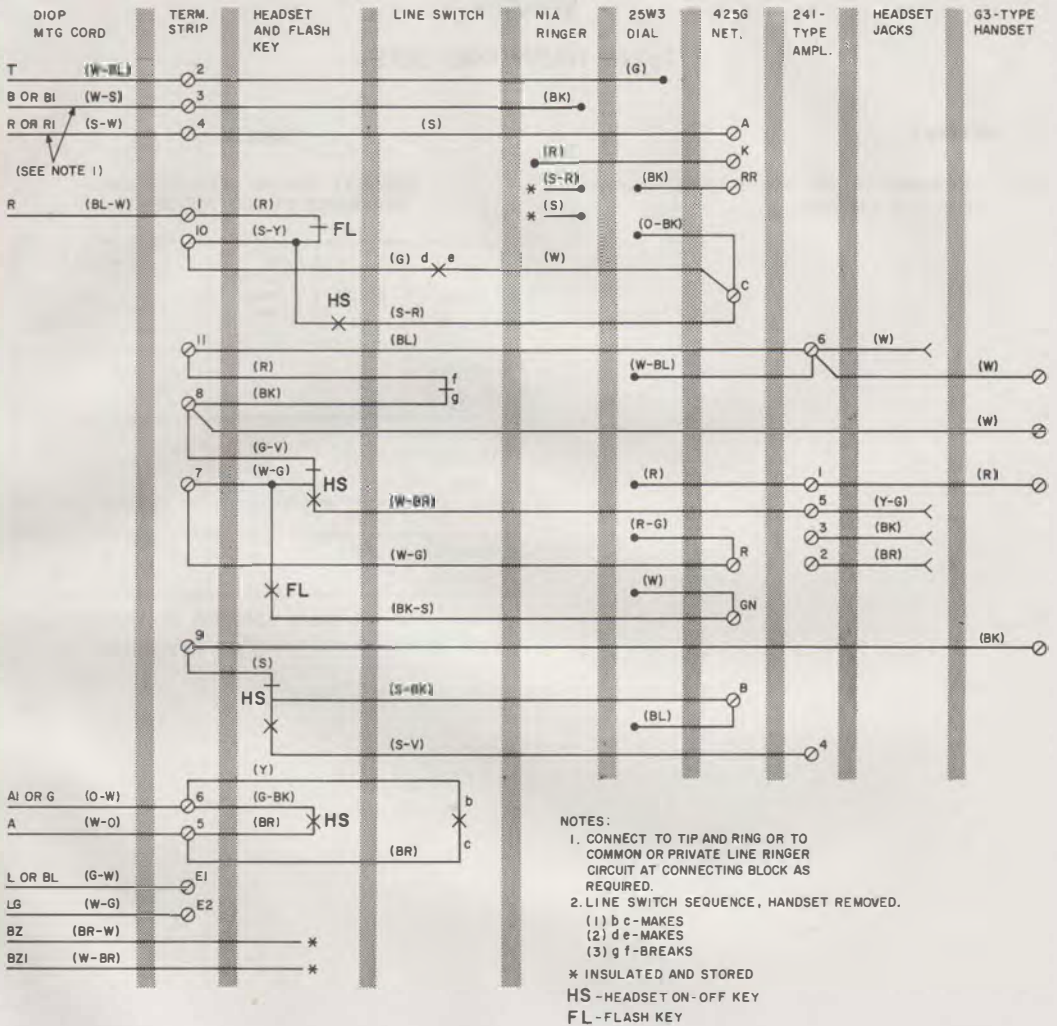
Fig. 1—1514B (MD) Telephone Set Connections With 25W3 (MD) Dial (Current Production)¶
