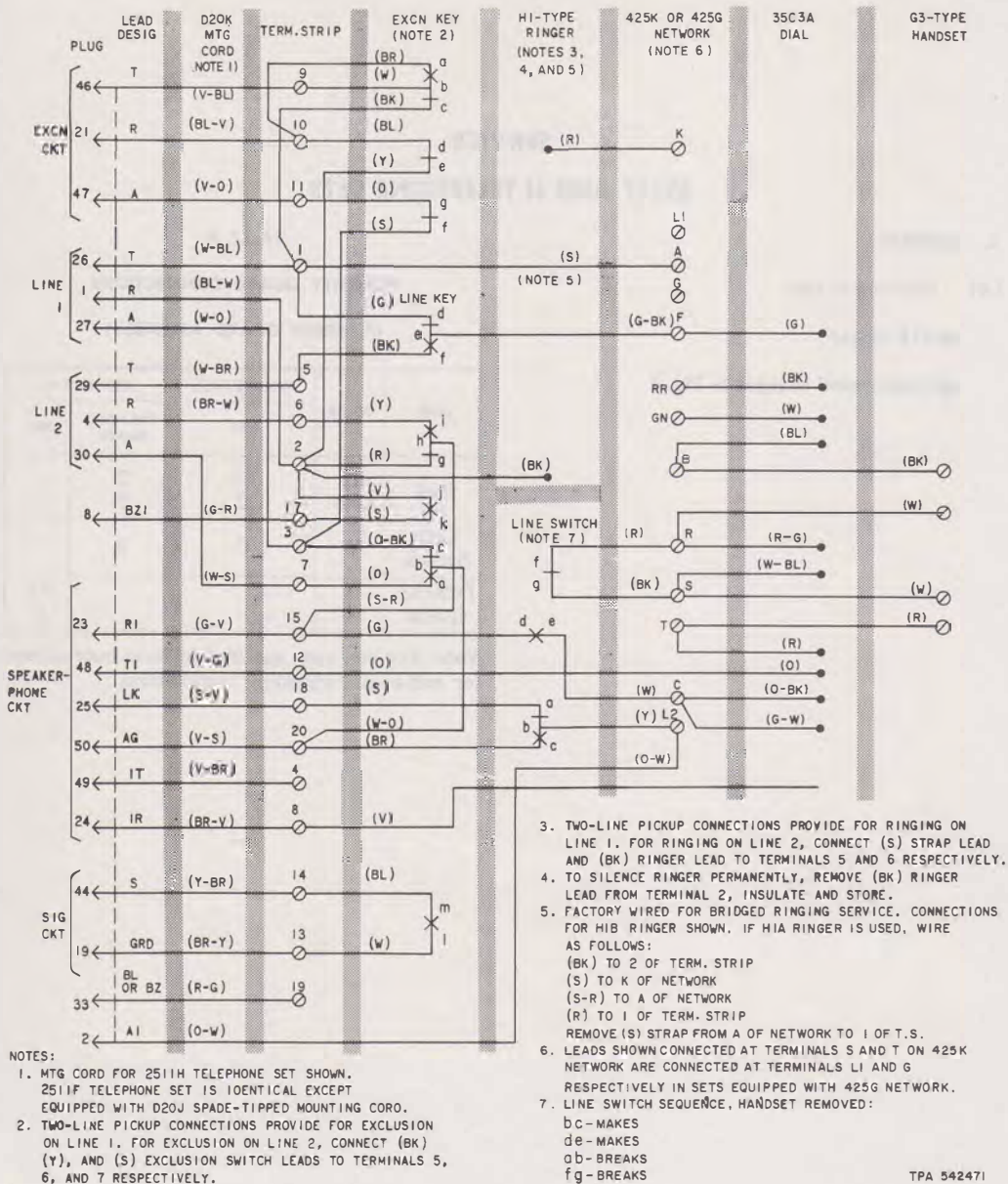
◆Fig. 1—2511F and H Telephone Sets, Connections (Factory Wired)◆
