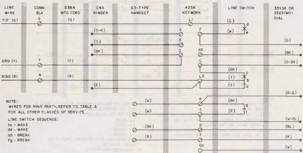
Fig. 1—2500D Telephone Set, Connections
