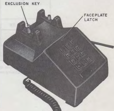
Fig. 1— 2503CM Telephone Set
