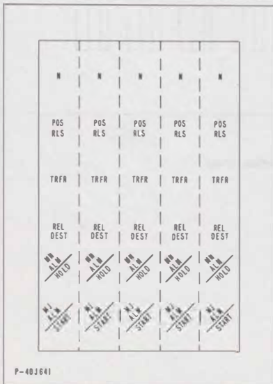
Fig. 11—P-40J641 Designation Strip
