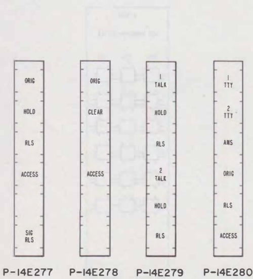
Fig. 3—Designation Strips
