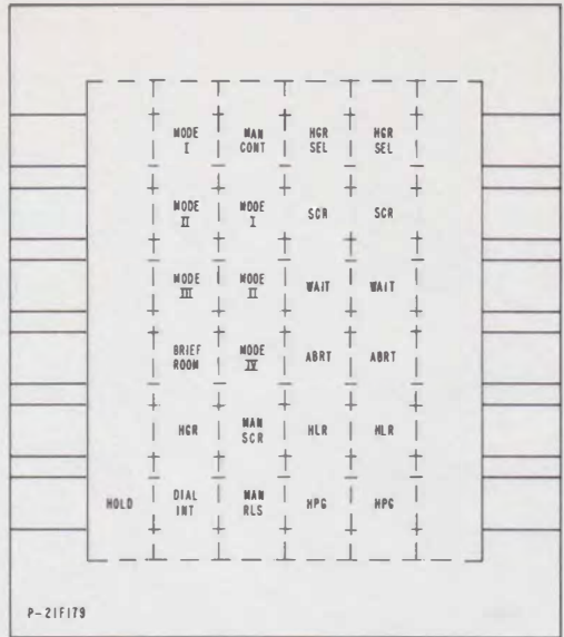
Fig. 8—P-21F179 Designation Strip
