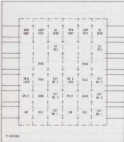
Fig. 7—P-44E509 Designation Strip
