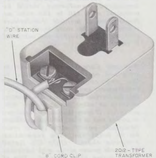
Fig. 3—Cord Clip Used to Secure Station Wire to Transformer
