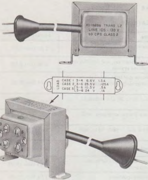
Fig. 8—KS-16886L2 Transformer
