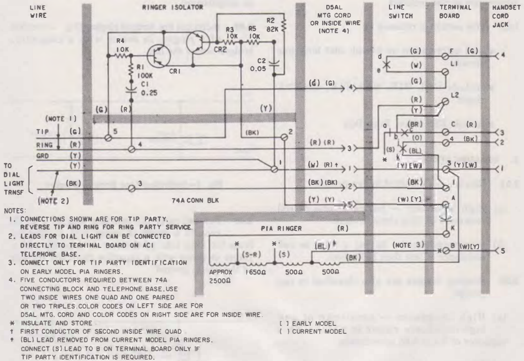
Fig. 9—74A Connecting Block and Ringer Isolator Connections with ACI or ADI Telephone Bases
