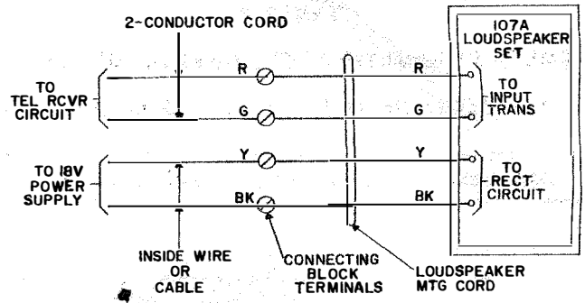
Fig. 3 - Loudspeaker Set, Connections
