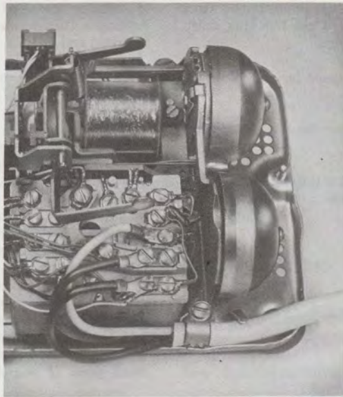
Fig. 5.1—Securing C Weatherproof Cord in Telephone Set
