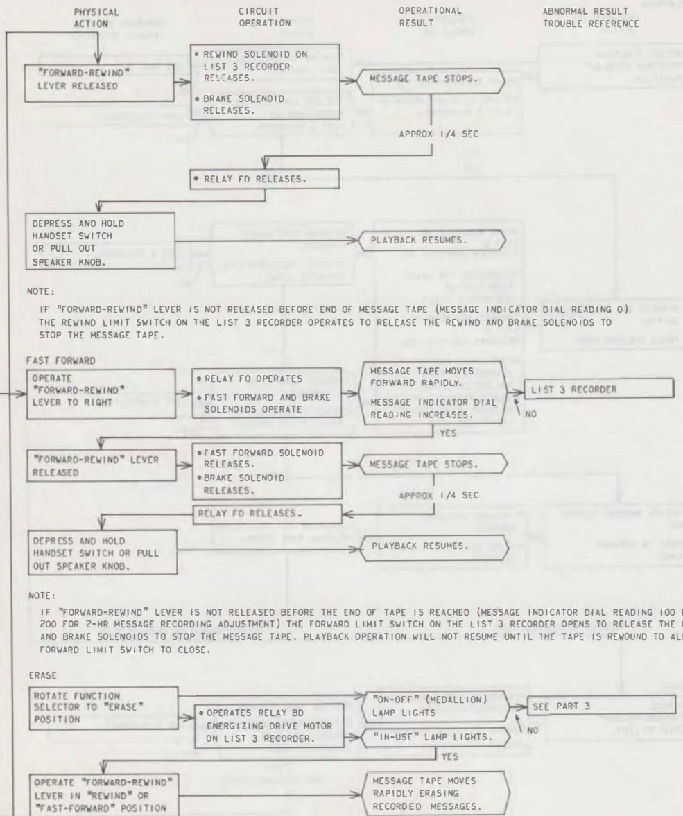
Fig. 10—Chart A (Sheet 10)
