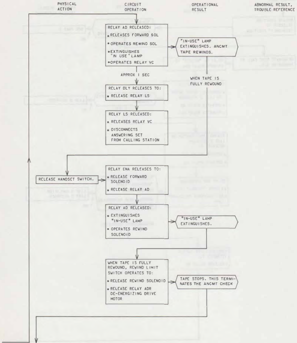
Fig. 10—Chart A (Sheet 4)
