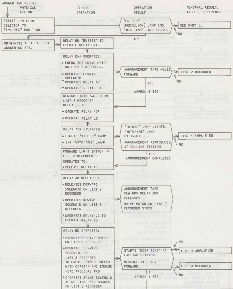
Fig. 11—Chart A (Sheet 7)
