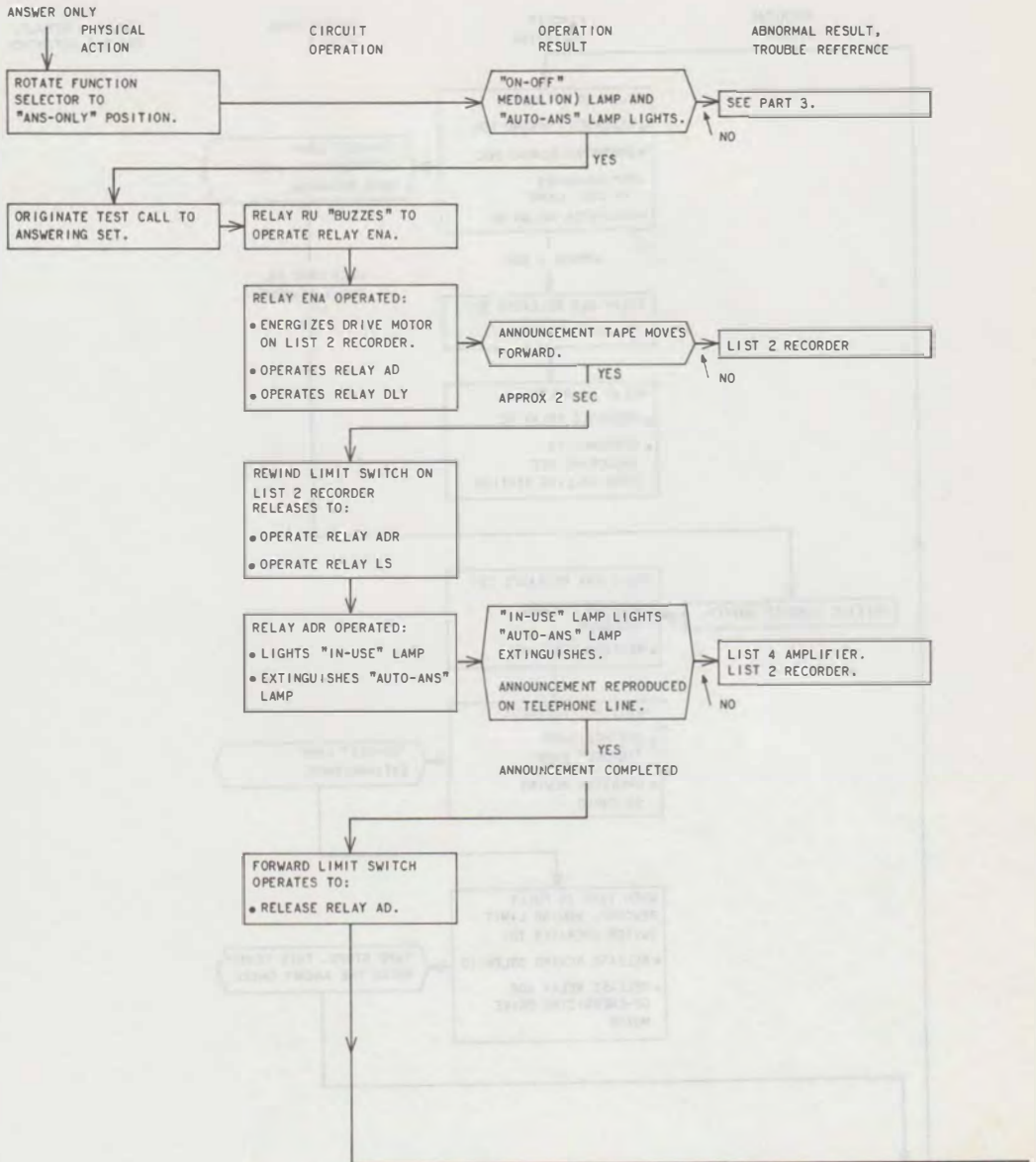
Fig. 10—Chart A (Sheet 3)
