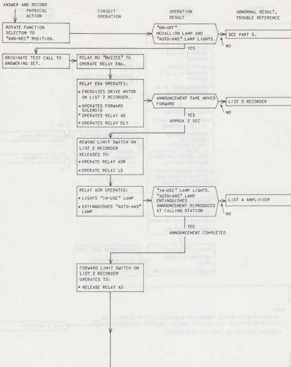
Fig. 10—Chart A (Sheet 5)
