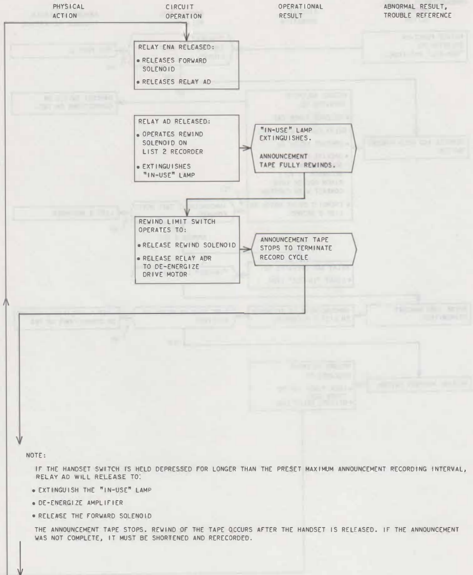
Fig. 10—Chart A (Sheet 2)
