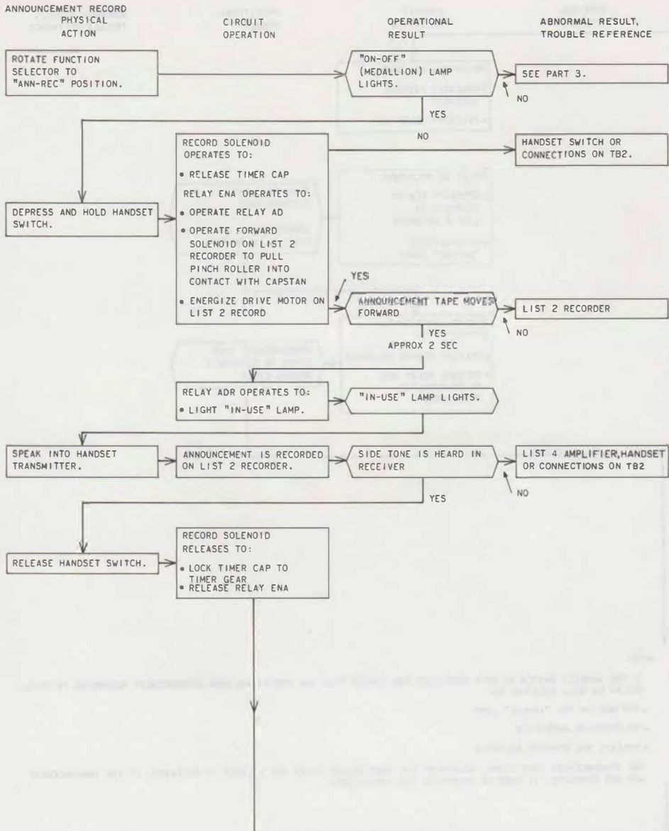
Fig. 10—Chart A (Sheet 1)
