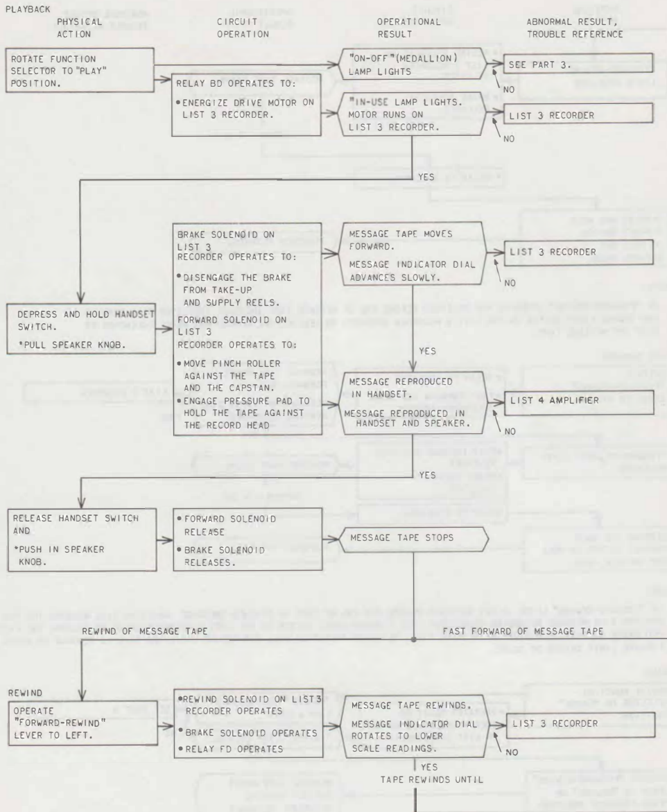
Fig. 12—Chart A (Sheet 9)
