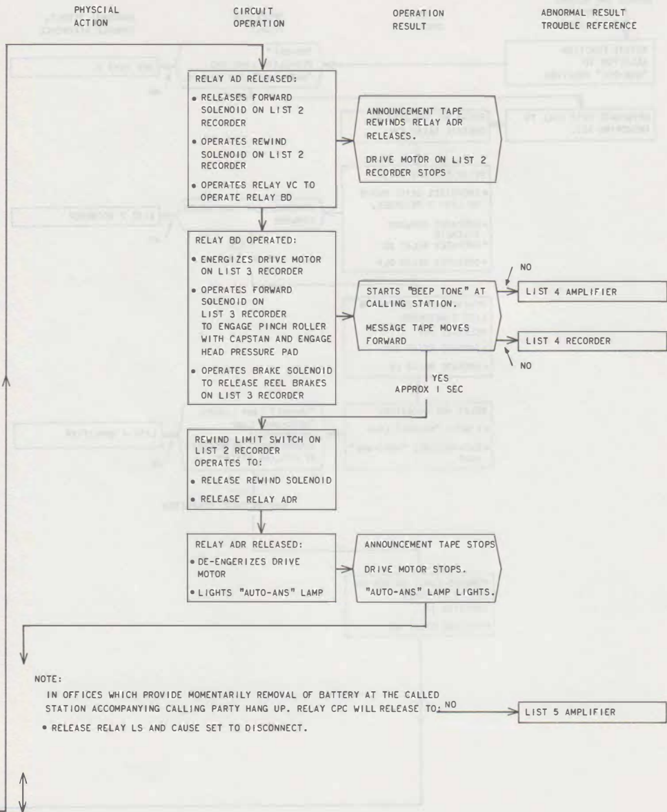
Fig. 10—Chart A (Sheet 6)
