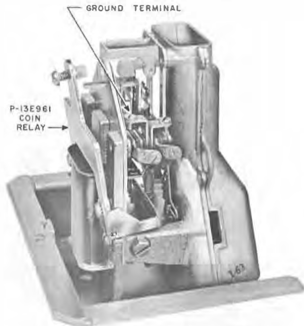
Fig. 35 — Manual or Dial Prepay, Single-Coil Slow-Release Coin Relay
