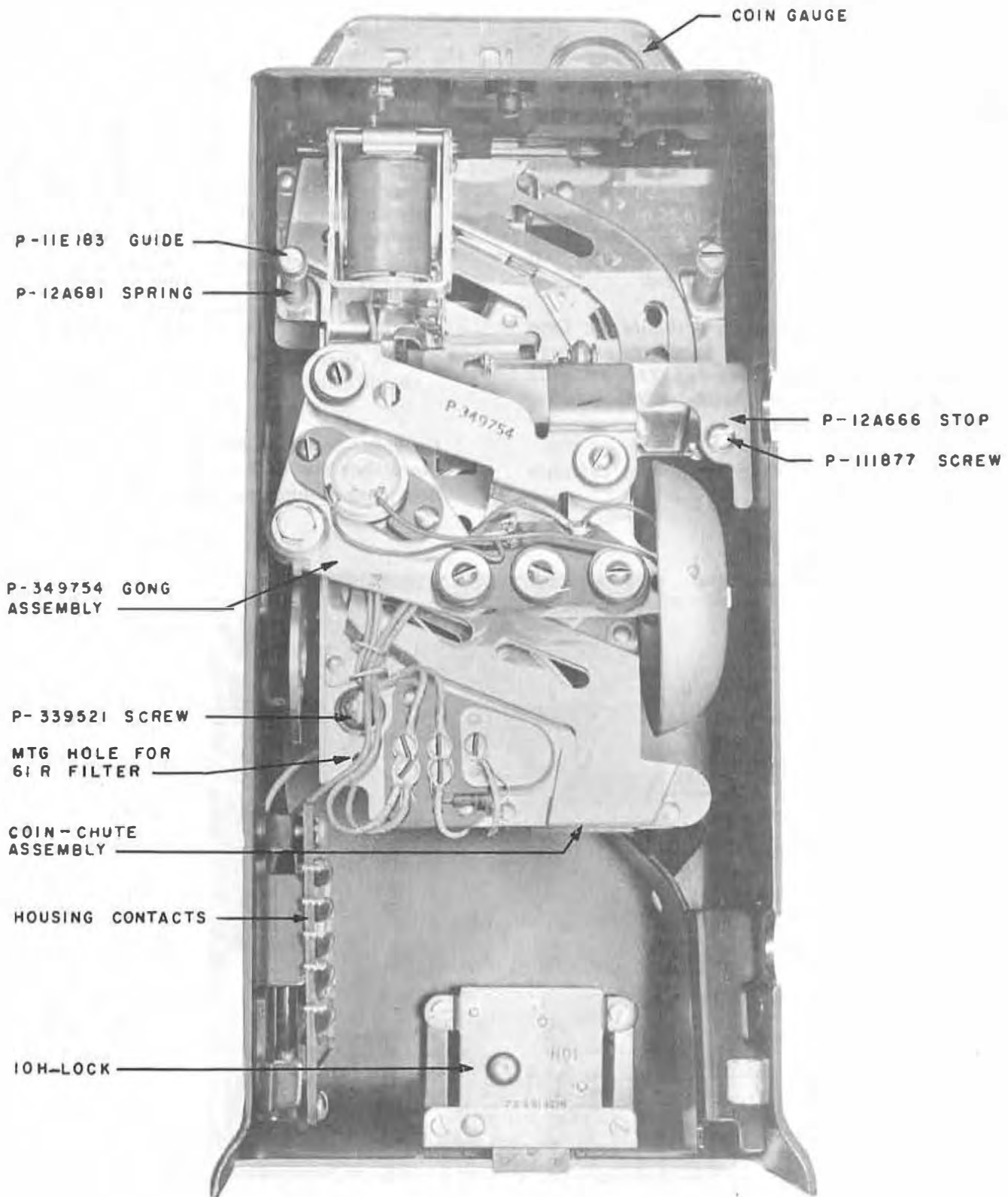
Fig. 8 - Upper Housing, Rear View
