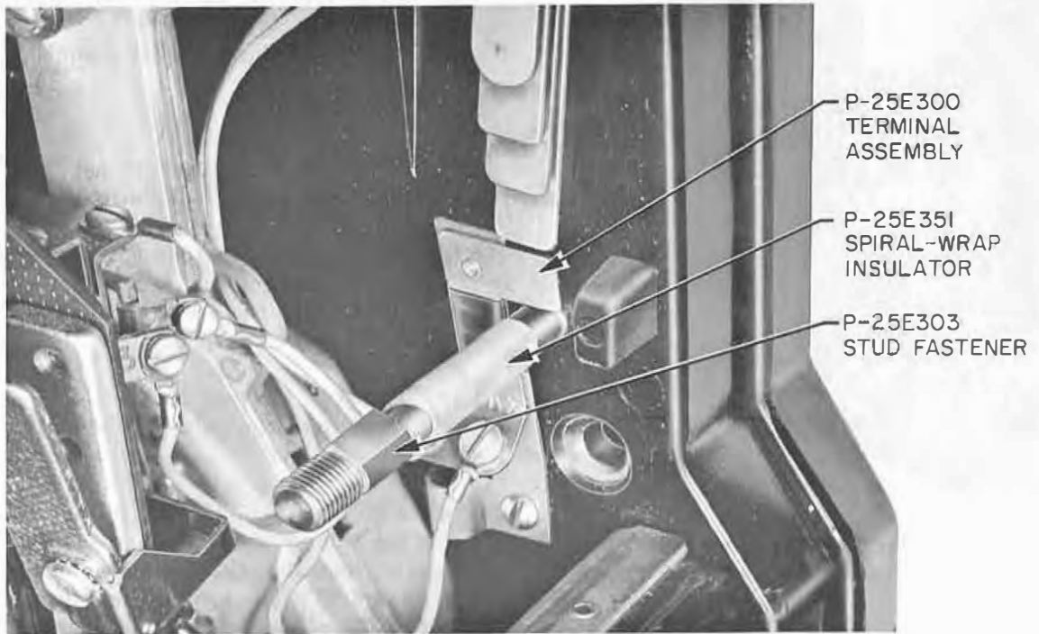
Fig. 22 — Terminal Assembly, Insulator, and Stud Fastener
