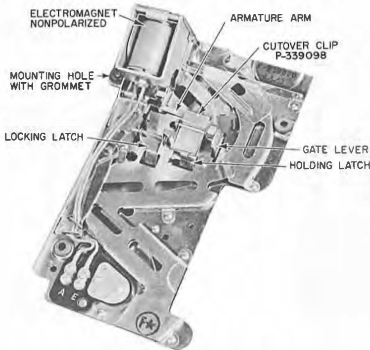
Fig. 15 — Prepay Coin Chute Equipped with Cutover Clip for 5-Cent Service
