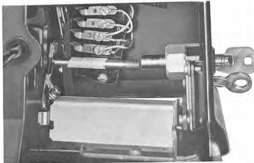
Fig. 27 — Cutaway Section of Upper Housing Showing Mating of Bolt Fastener and KS-19277 Lock with Housing Placed on Coin Collector
