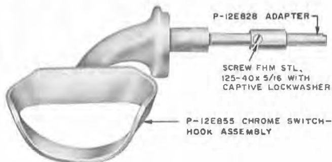
Fig. 31 — 2-Piece Switchhook Assembly
