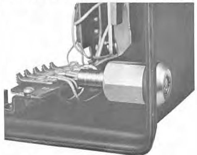
Fig. 19—Cutaway Section of Upper Housing, KS-19277 Lock Assembly Installed
