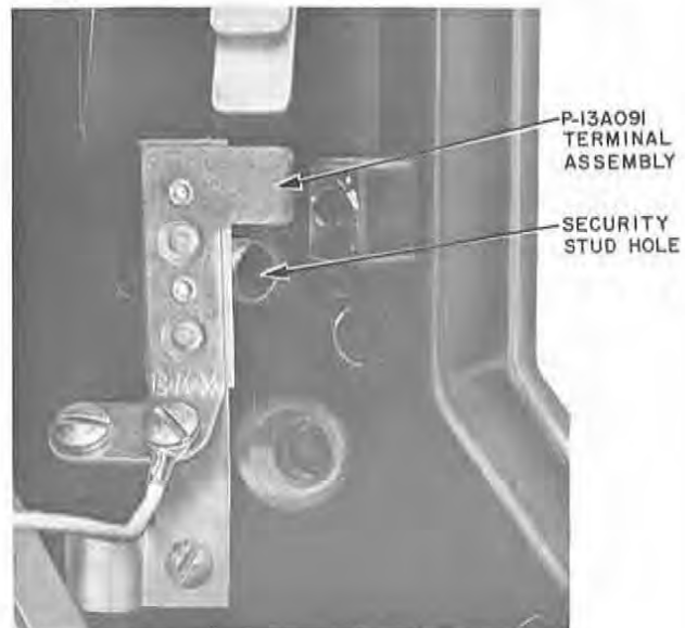
Fig. 21 — P-13A091 Terminal Assembly and Vacant Security Stud Hole
