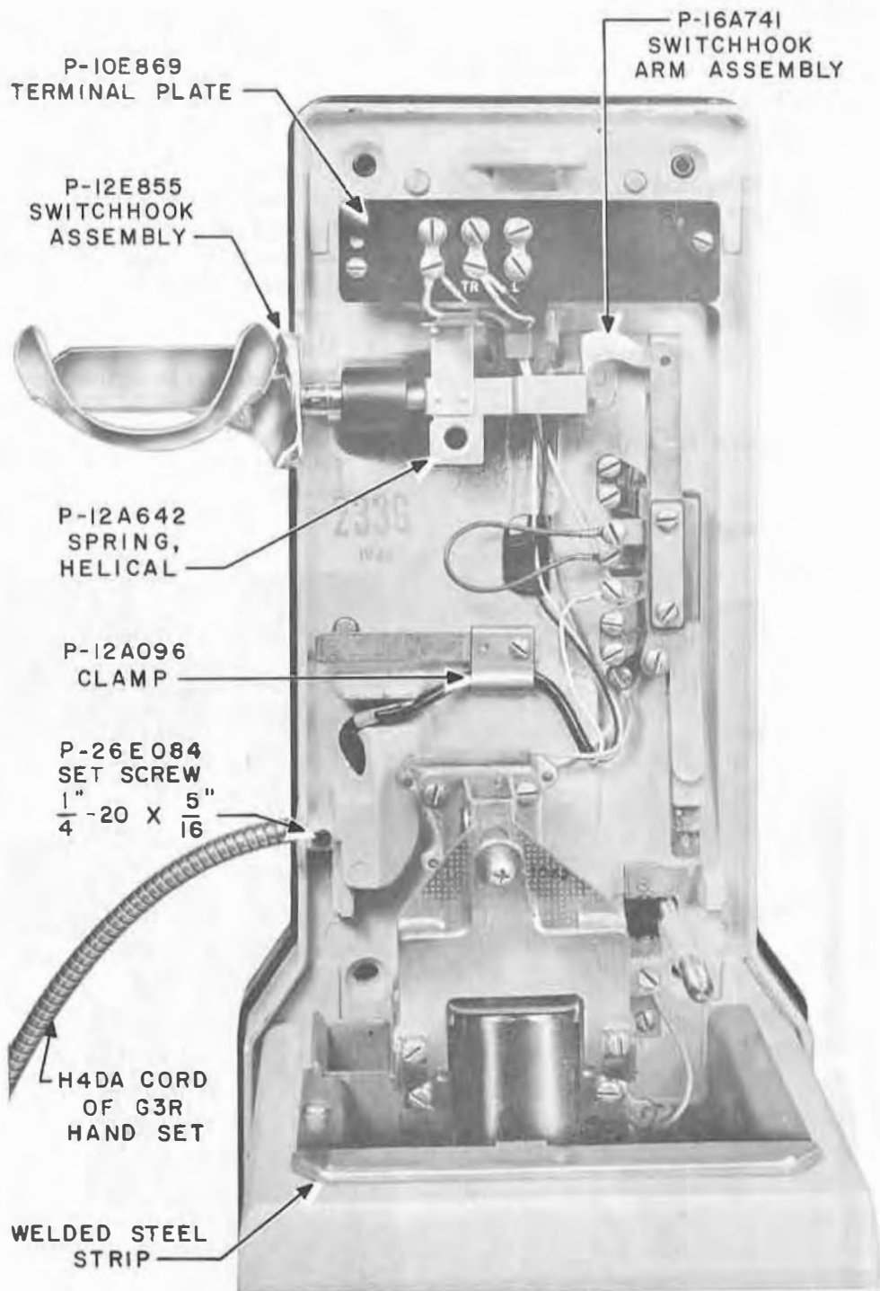
Fig. 4—Typical Backplate Assembly
