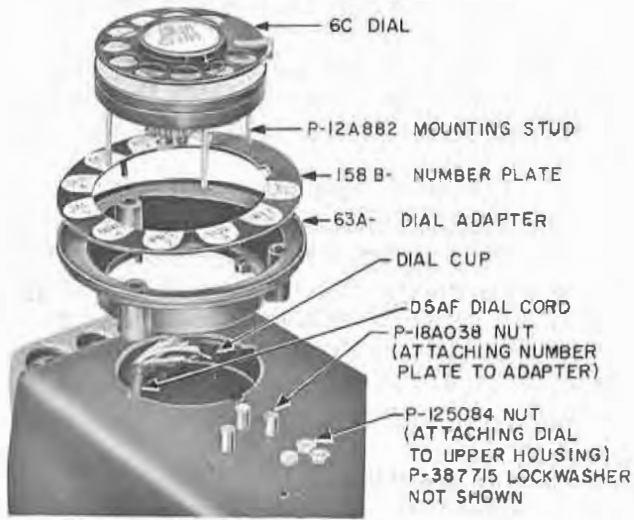
Fig. 10 - Assembly of 6-Type Dial
