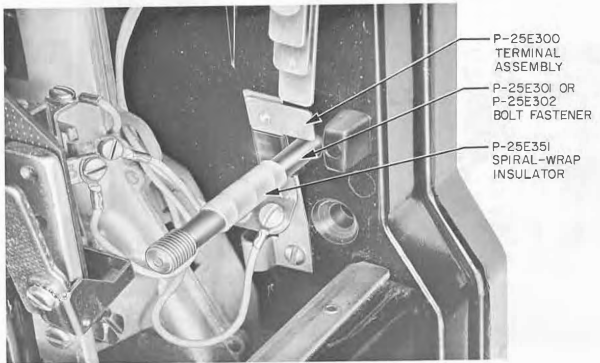
Fig. 23 — Terminal Assembly, Bolt Fastener, and Insulator
