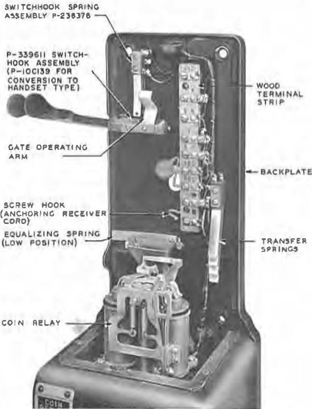
Fig. 2—Earlier Type Coin Collector with Wood Terminal Strip
