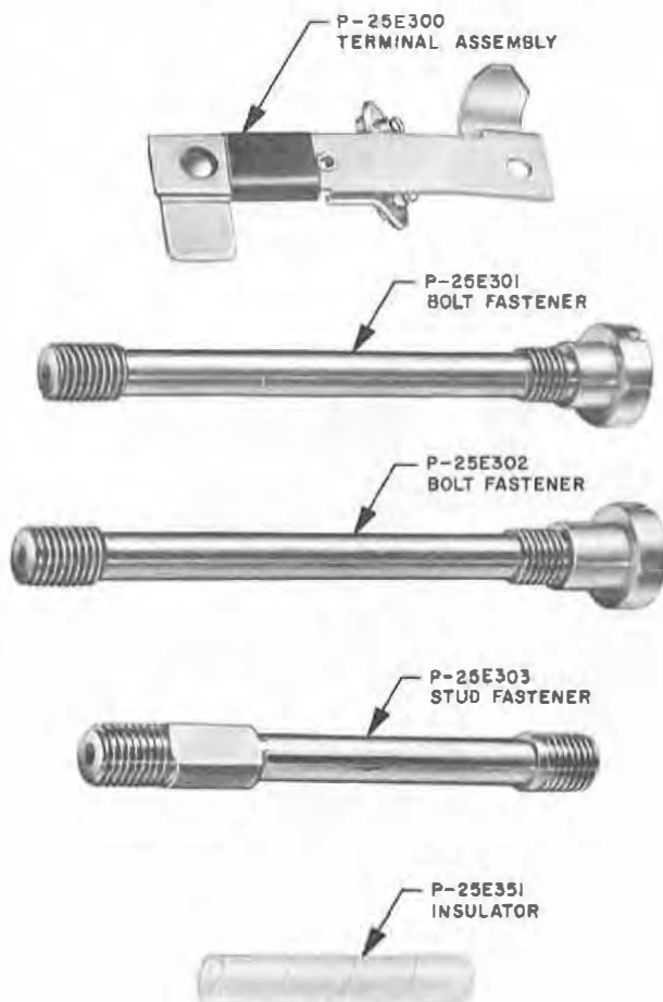
Fig. 17—Terminal Assembly, Associated Fasteners, and Insulator
