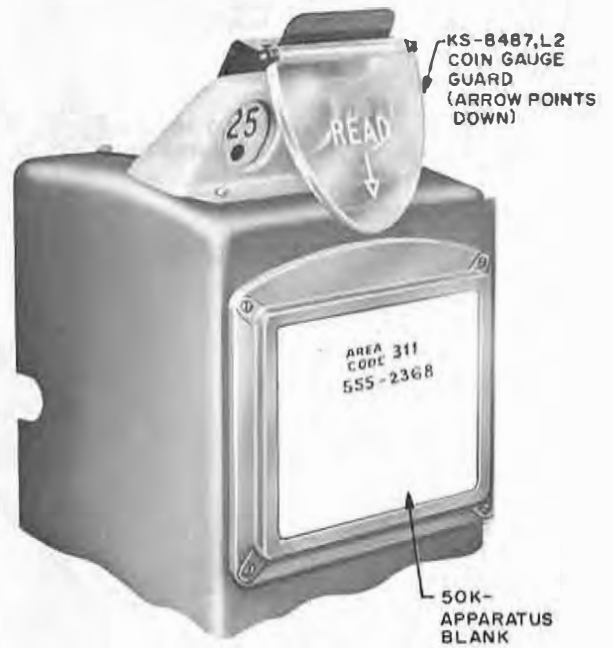
Fig. 13 - Manual Postpay Coin Collector Equipped with Coin Gauge Guard
