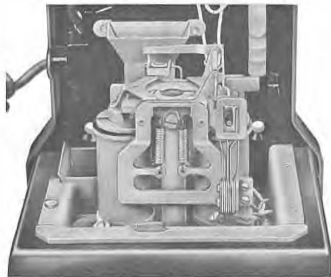
Fig. 34 — Manual or Dial Prepay, 2-Coil Coin Relay
