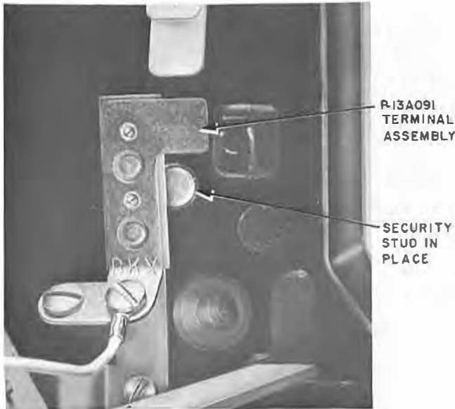
Fig. 24 — Terminal Assembly and Security Stud Installed
