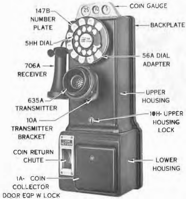
Fig. 11 - Transmitter Receiver Type Coin Collector
