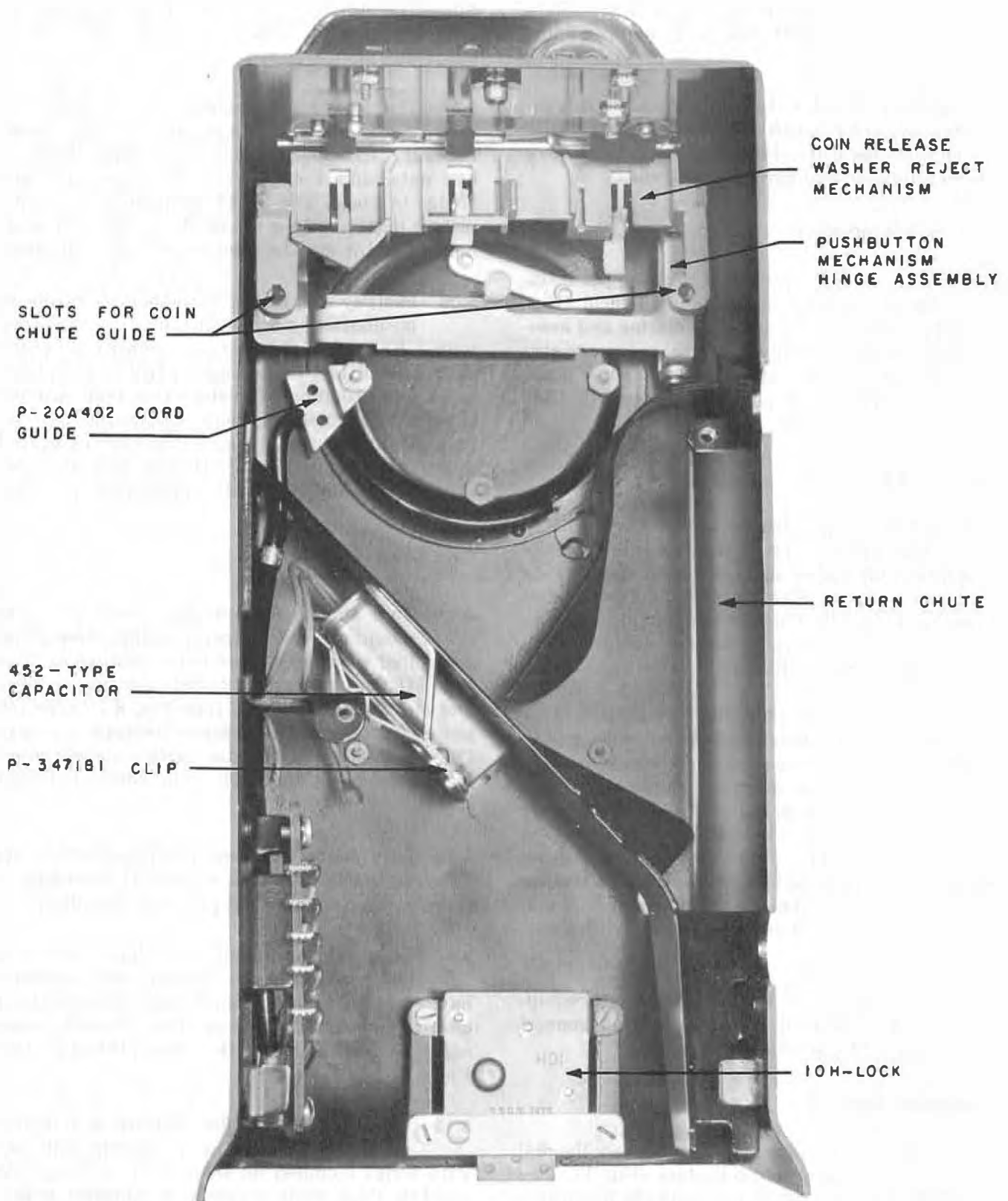
Fig. 9 - Upper Housing, Interior View
