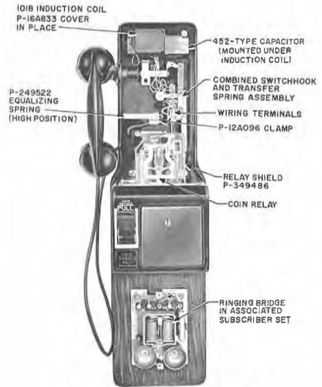
Fig. 3—Combined Assembly with Induction Coil and Capacitor
