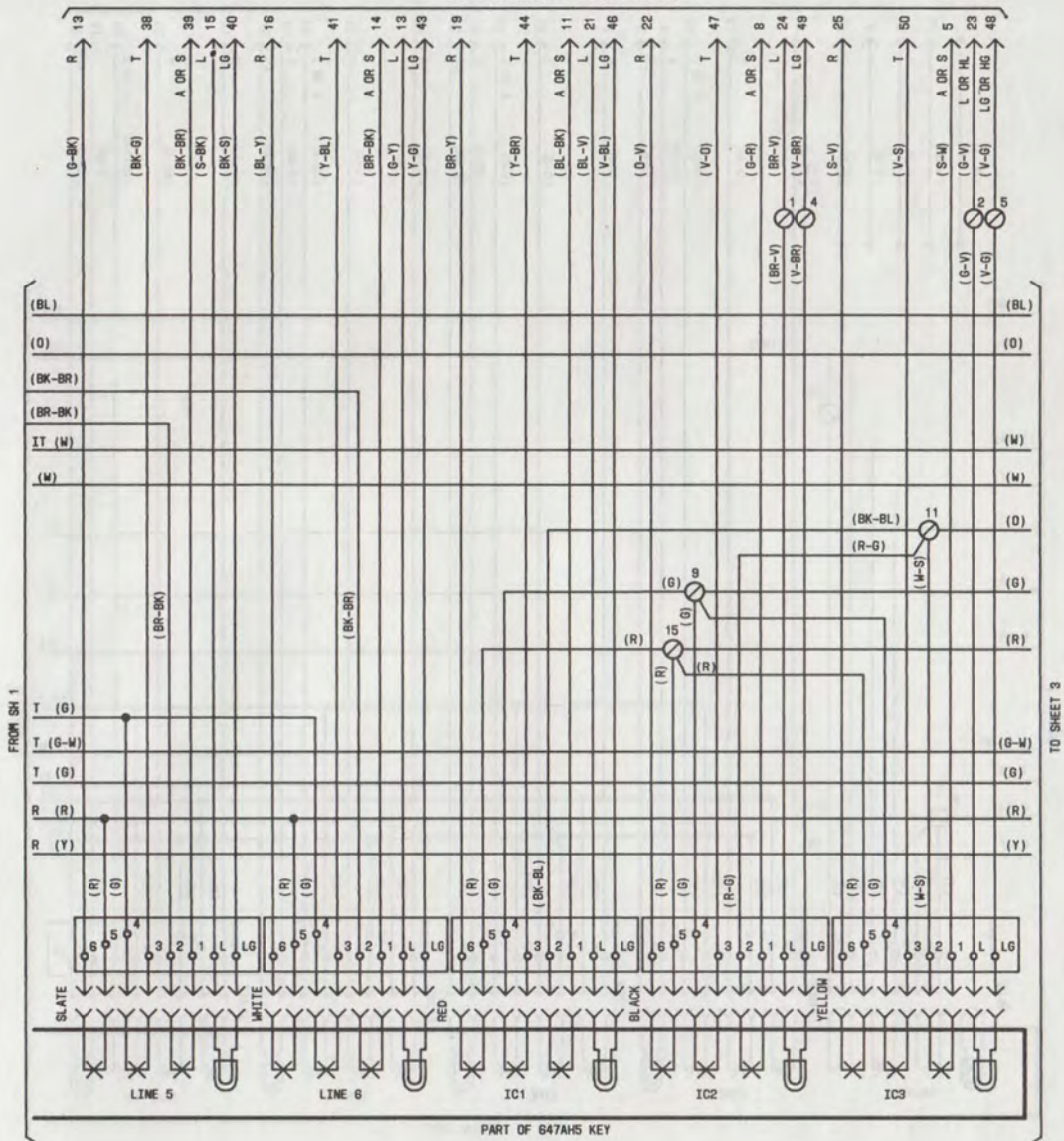
Fig. 14—831FM or 2831FM Telephone Set, Key and Mounting Cord Arrangement (Sheet 2 of 4)
