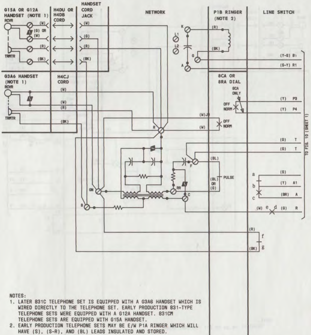
Fig. 5—Part of 831A1M (MD), B1M (MD), C (MD), CT (MD), or CM (Equipped With Old Line Switch) Telephone Set, Connections
