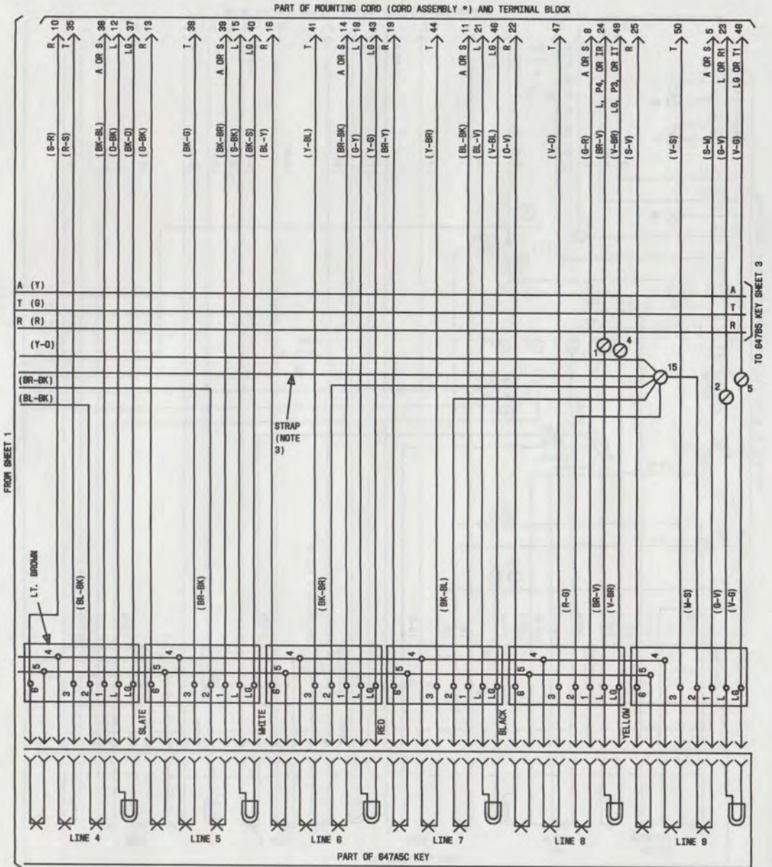
Fig. 10—831A1M (MD), B1M (MD), C (MD), CT (MD), CM or 2831A1M (MD), B1M (MD), C (MD), CT (MD), CM Telephone Set, Key and Mounting Cord Arrangement (Sheet 2 of 4)
