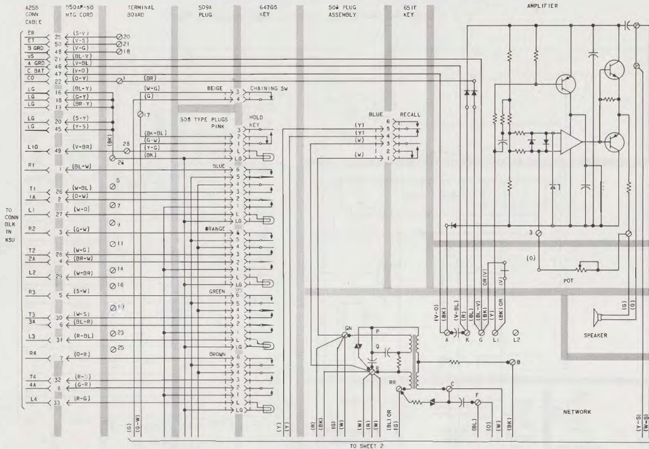
Fig. 10—832BM or 832DM Telephone Set, Connections (Sheet 1 of 2)
