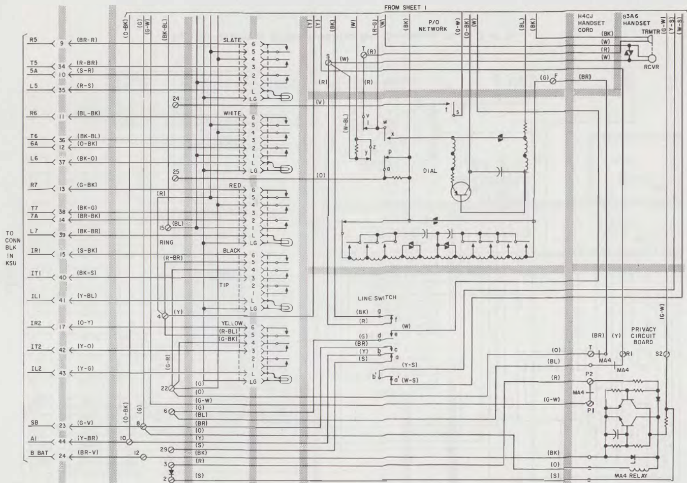
Fig. 13—2832C (MD) Telephone Set, Connection (Sheet 2 of 2)
