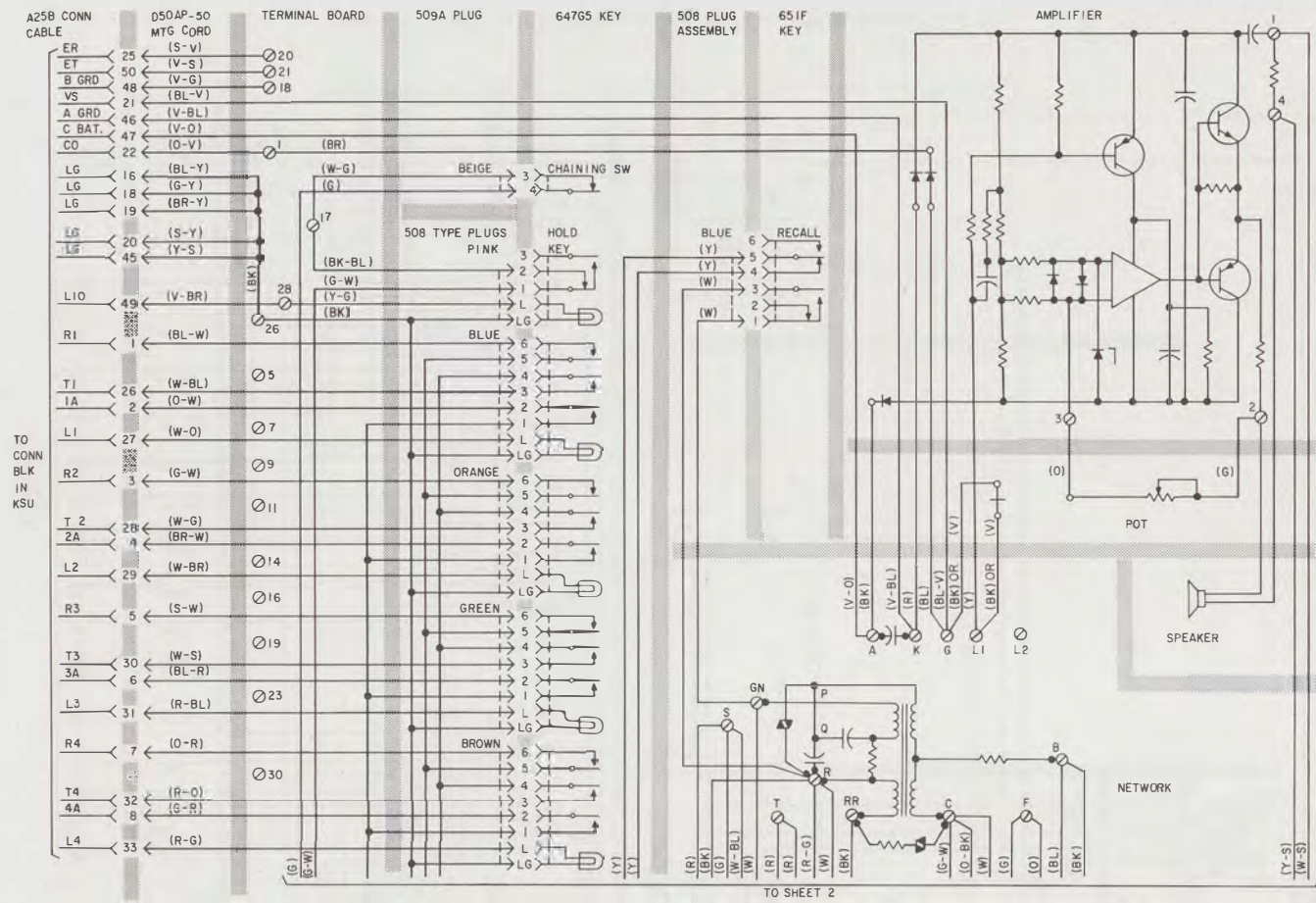
Fig. 11—2832BM or 2832DM Telephone Set, Connections (Sheet 1 of 2)
