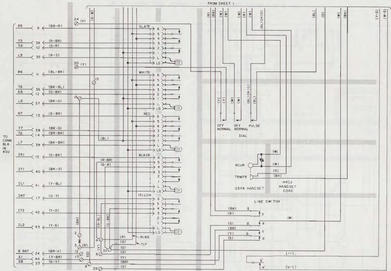
Fig. 6-832A (MD) Telephone Set, Connections (Sheet 2 of 2)
