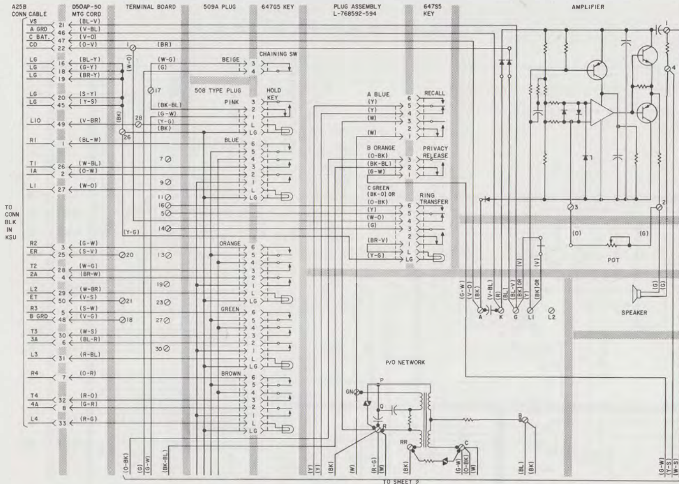
Fig. 13—2832C (MD) Telephone Set, Connections (Sheet 1 of 2)
