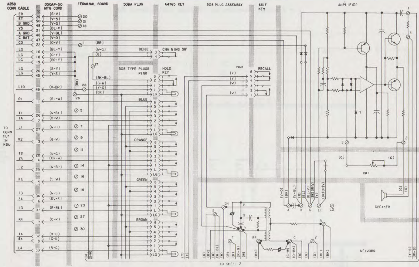
Fig. 9—2832B (MD) Telephone Set, Connections (Sheet 1 of 2)
