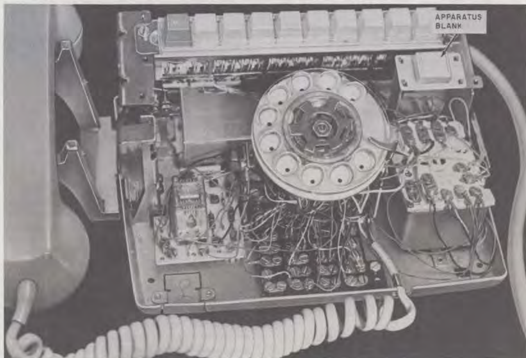
Fig. 3—832A Telephone Set (Housing Removed)
