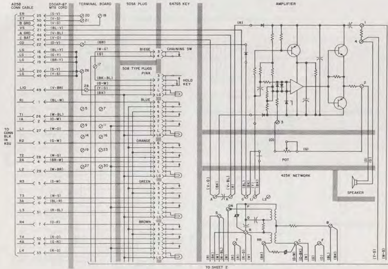
Fig. 6—2832A Telephone Set, Connections (Sheet 1 of 2)
