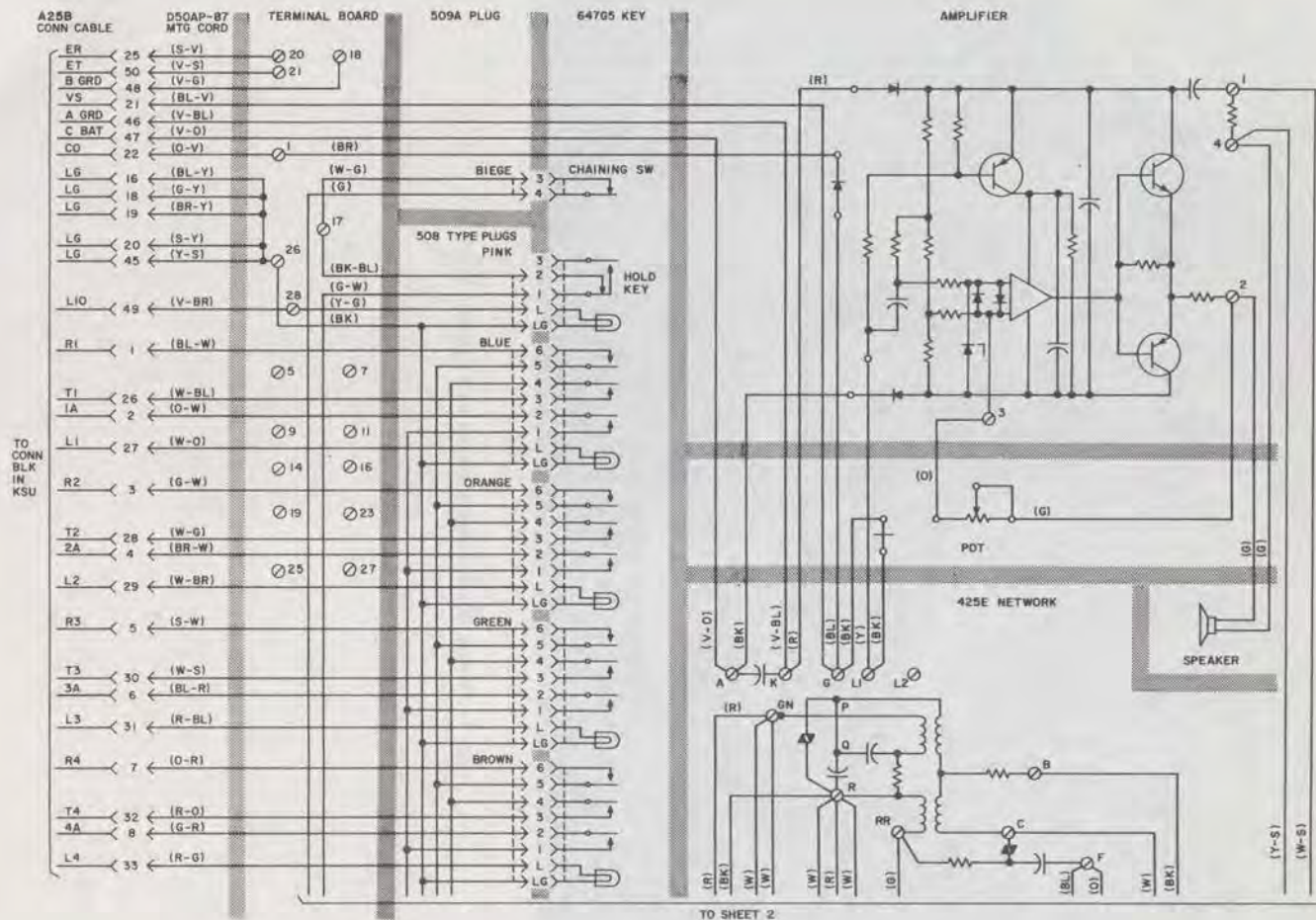
Fig. 5—832A Telephone Set, Connections (Sheet 1 of 2)
