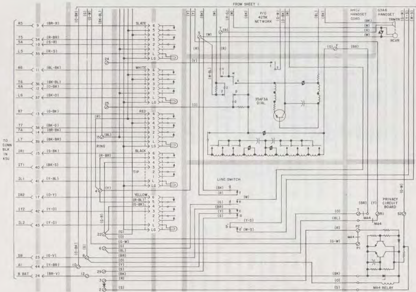
Fig. 10—2832C Telephone Set, Connections (Sheet 2 of 2)
