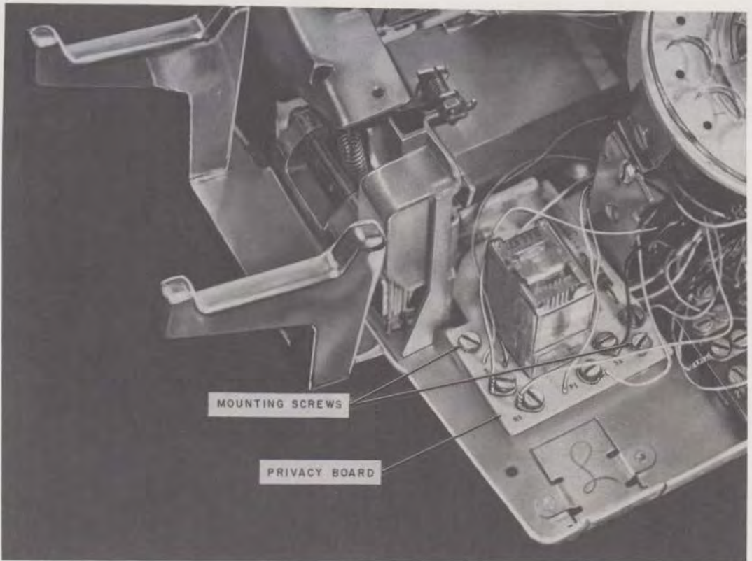
Fig. 4—Privacy Circuit Board Mounted on Telephone Set
