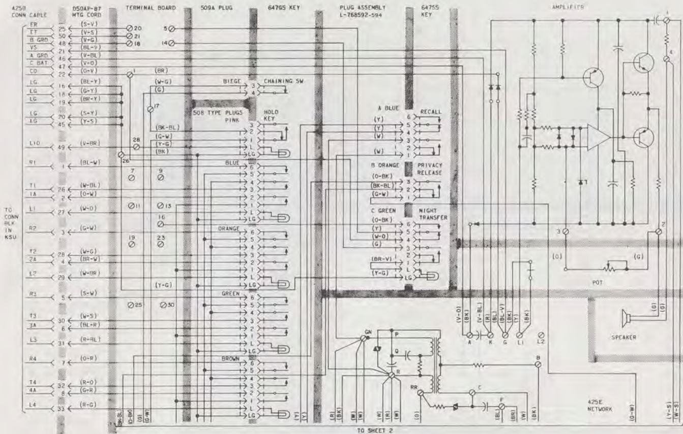
Fig. 9—832C Telephone Set, Connections (Sheet 1 of 2)
