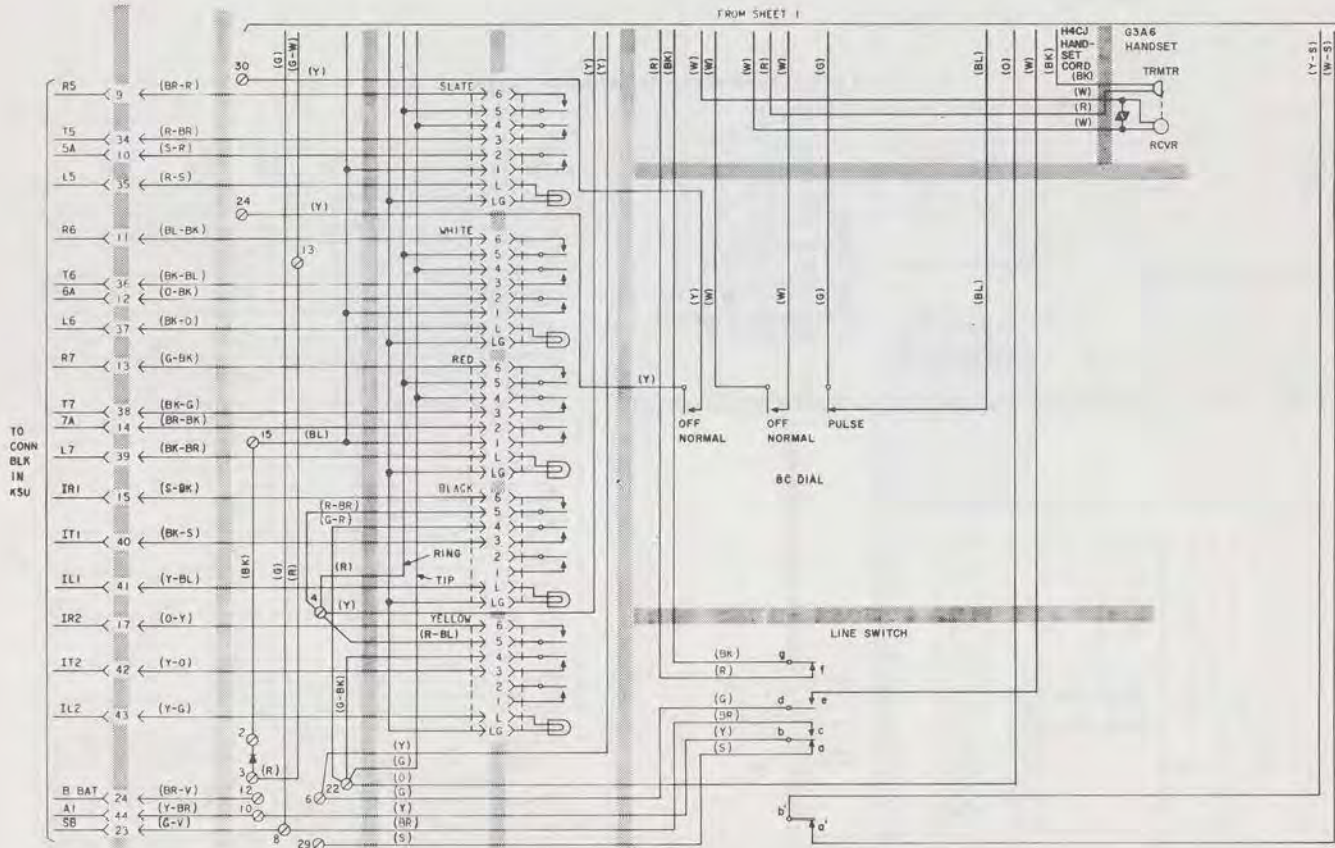
Fig. 7—832B Telephone Set, Connections (Sheet 2 of 2)
