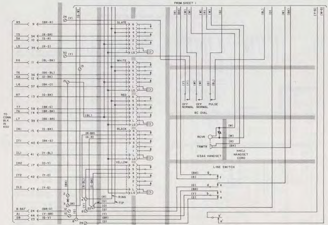
Fig. 5—832A Telephone Set, Connections (Sheet 2 of 2)
