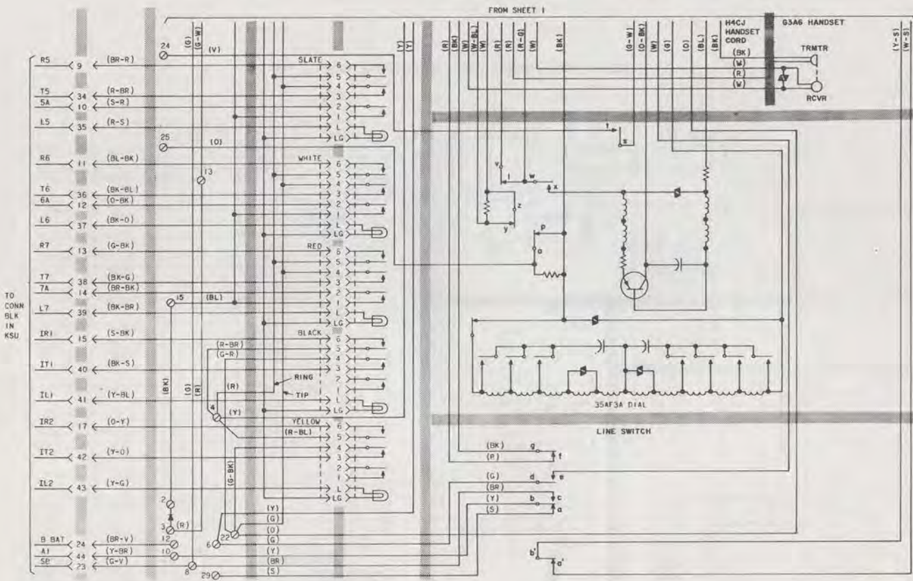
Fig. 8—2832B Telephone Set, Connections (Sheet 2 of 2)
