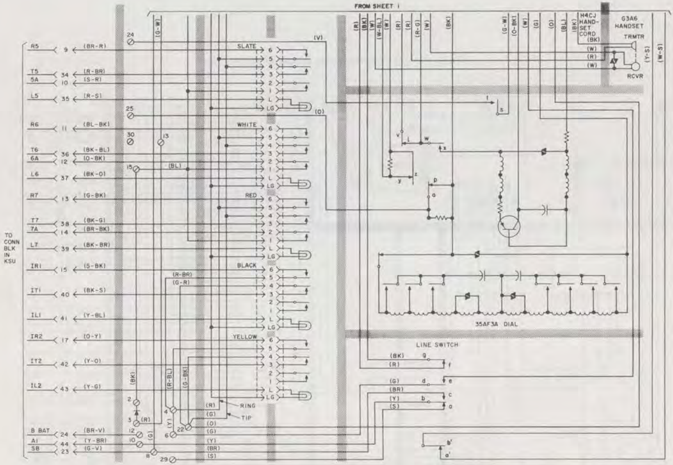
Fig. 6—2832A Telephone Set, Connections (Sheet 2 of 2)
