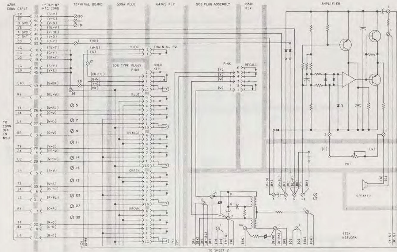
Fig. 8—2832B Telephone Set, Connections (Sheet 1 of 2)
