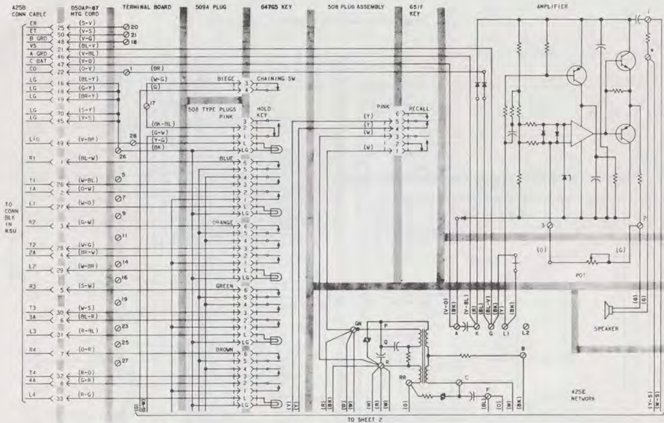
Fig. 7—832B Telephone Set, Connections (Sheet 1 of 2)
