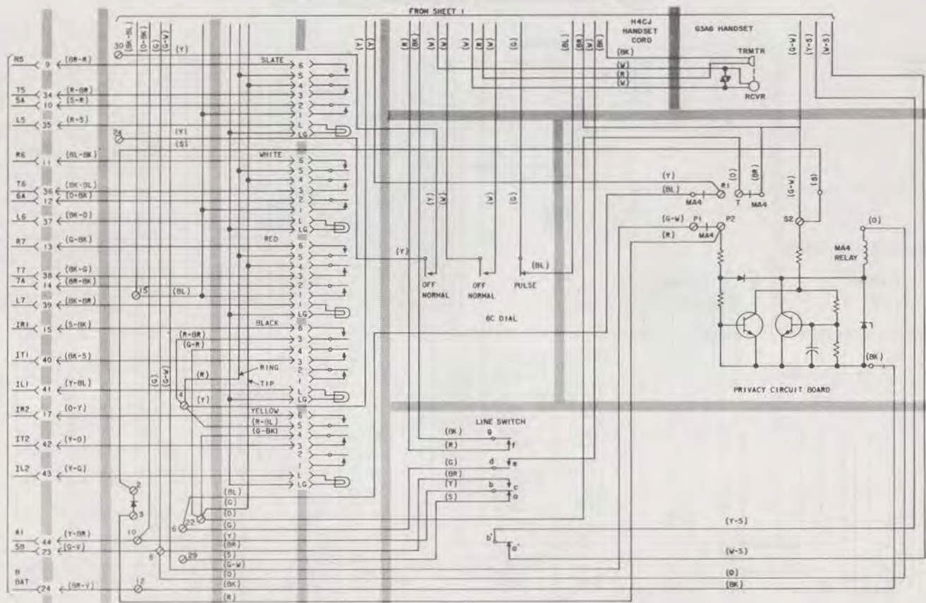
Fig. 9—832C Telephone Set, Connections (Sheet 2 of 2)
