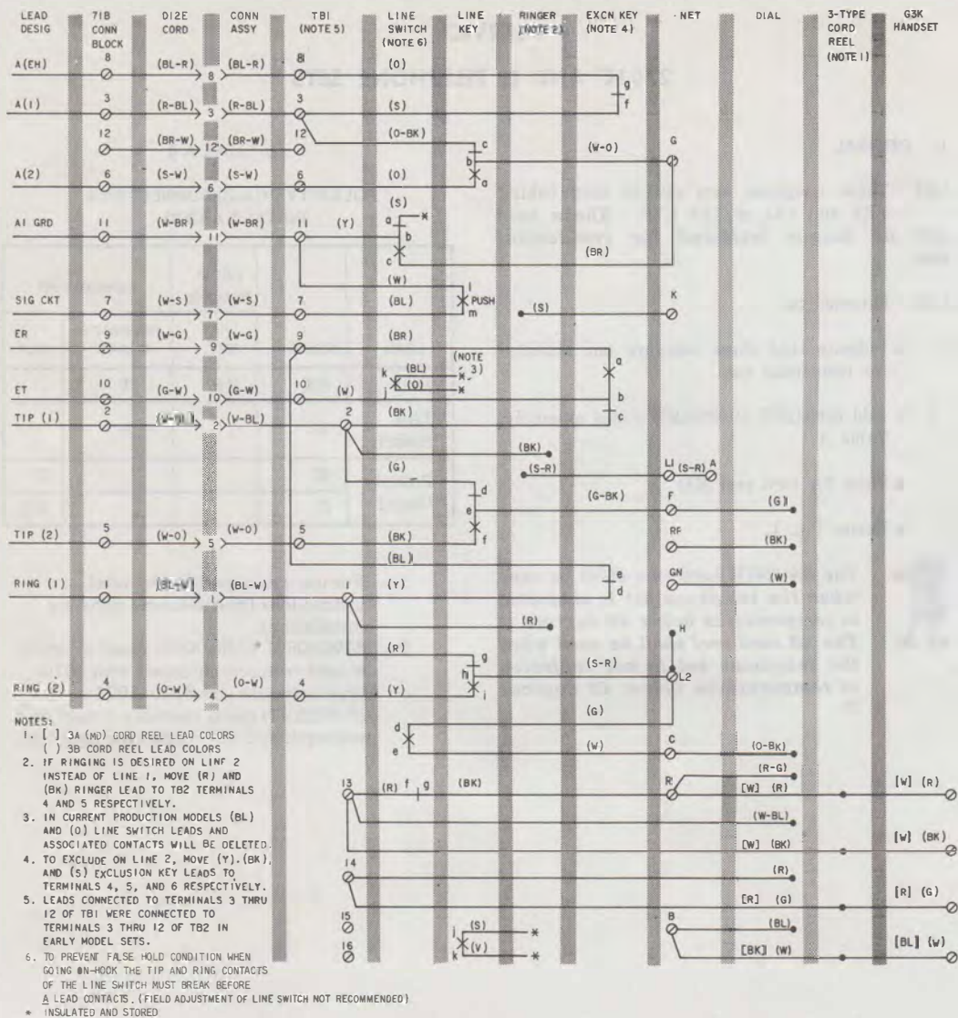
Fig. 1—2751C and D Telephone Sets, Connections
