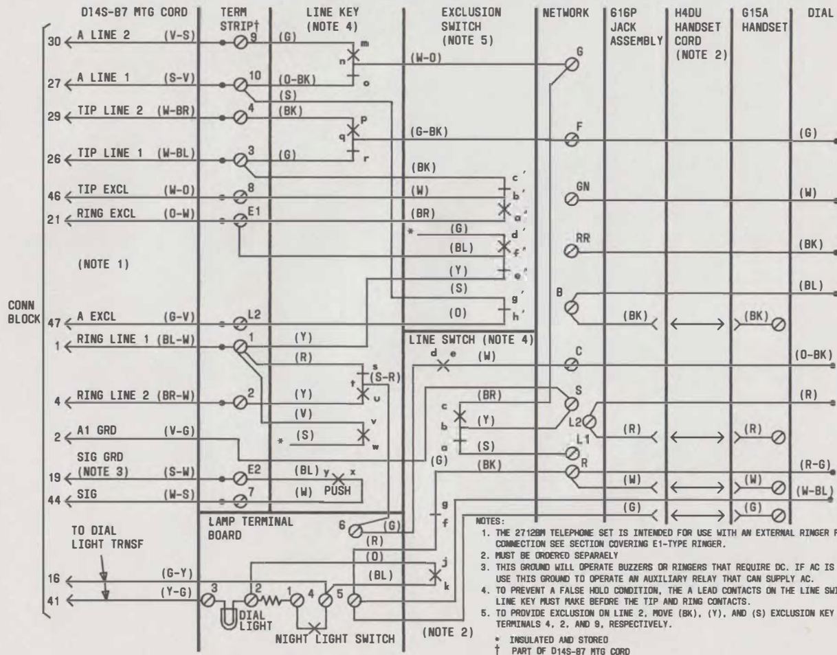
Fig. 2—2712BM Telephone Set Connections, 2-Line Pickup, Exclusion on Line 1, and Signaling (Used with 1A1 or 1A2 KTS) (Factory Wiring)
