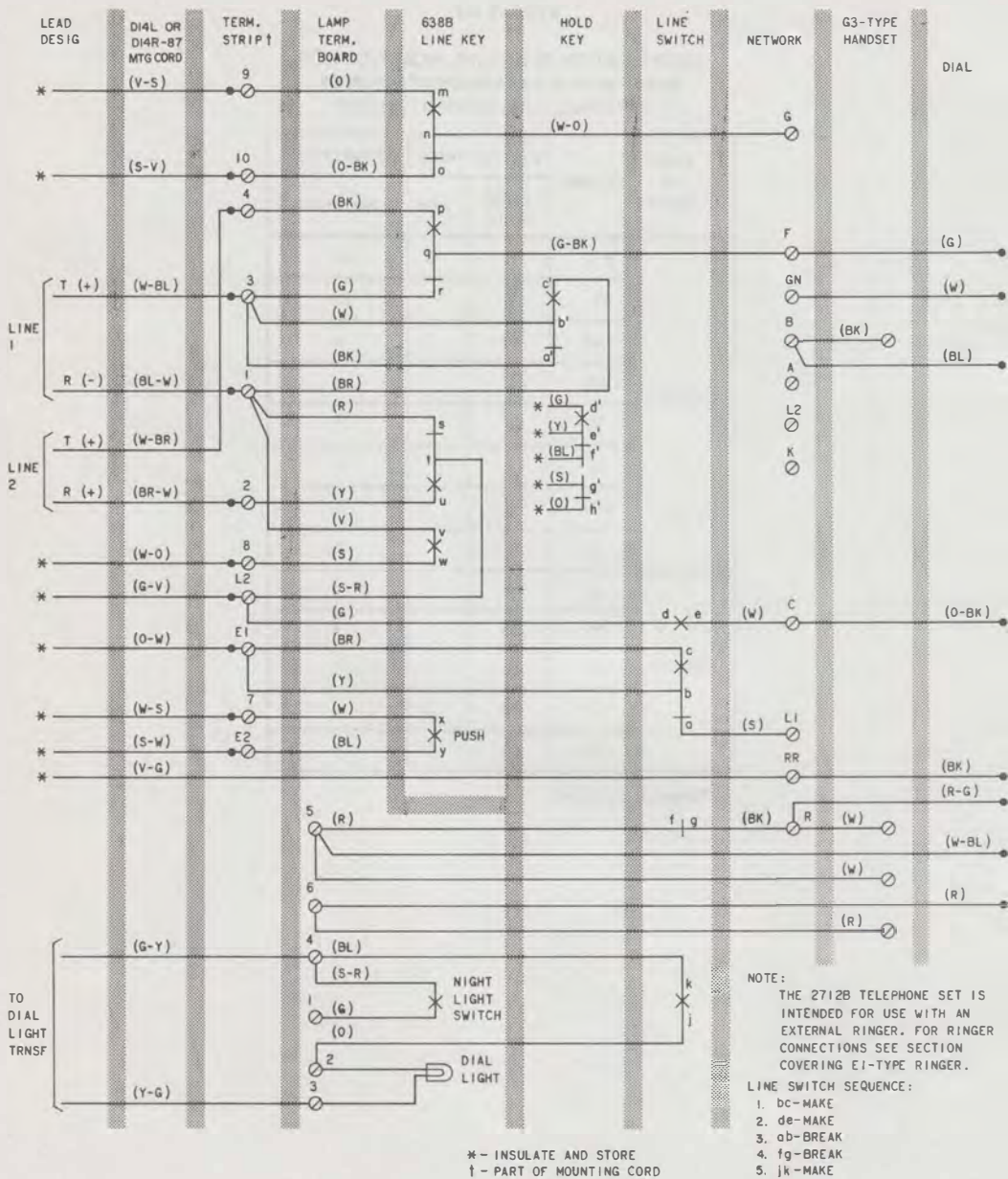
Fig. 1—2712B Telephone Set Connections, 2-Line Pickup with Hold on Line 1 (Factory Wiring)
