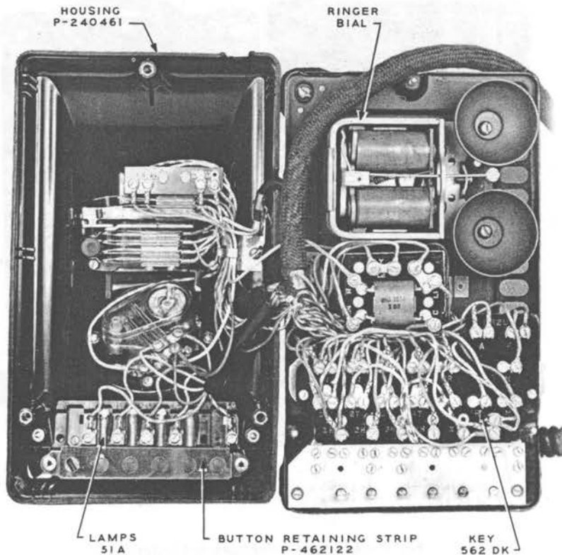
Fig. 6 - 465-type Telephone Set (Internal)
