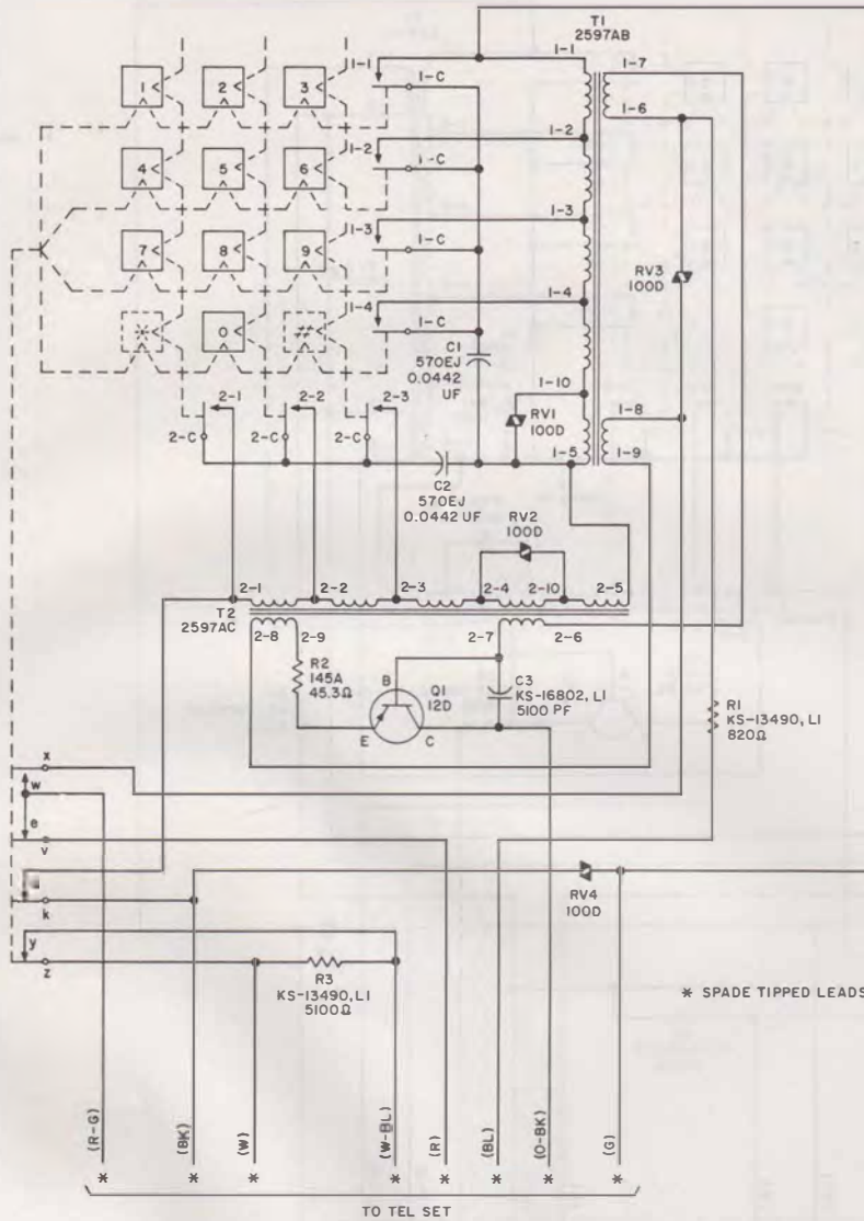
Fig. 18—25P4 and 25W3 Dials, Schematic
