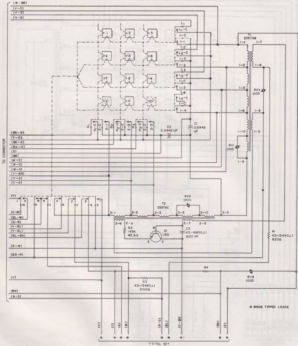
Fig. 22-25U3 Dial, Schematic
