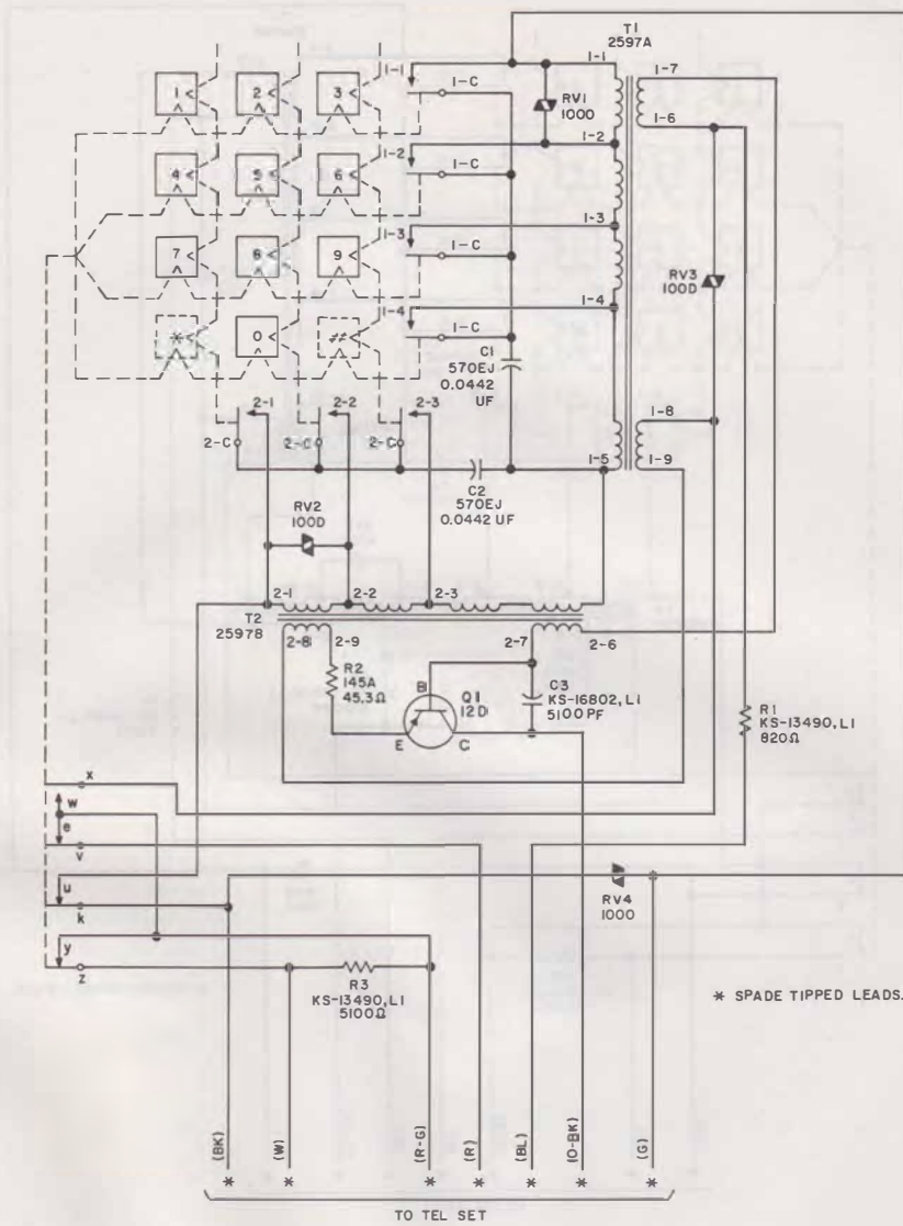
Fig. 10—25A3 and 25H4 Dials (MD), Schematic
