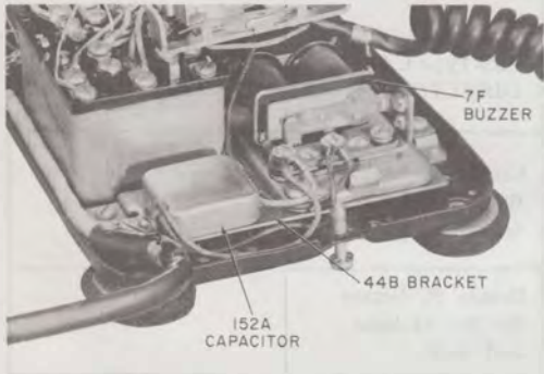
Fig. 13—7F Buzzer and 152A Capacitor Mounted on 44B Bracket
